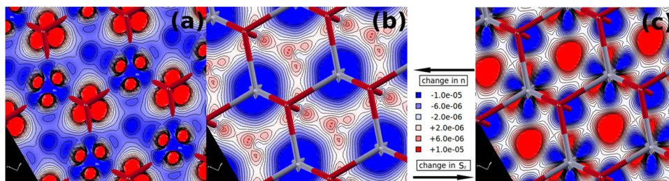
Fig. 5 Computed photoinduced changes in charge and spin density in FeRh. a, b Changes in the charge density n(\mathbf{r}, t_f) - n^{\text{eq}}(\mathbf{r}) and (c) spin density S_z(\mathbf{r}, t_f) - S_z^{\text{eq}}(\mathbf{r}) at the end of the laser pulse ( t = t_f ) with respect to the equilibrium configuration. Densities are in atomic units ( [e/a_0^3] and [\mu_B/a_0^3] , where a_0 = 5.29 \times 10^{-11} m is the Bohr radius. 0.25 electron per unit cell corresponds to a density of 7 \times 10^{-4} e/a_0^3 .) on two different FeRh[111]-planes: the plane just below the Fe( \uparrow ) atoms ( a ) and the plane containing the Rh atoms ( b, c ). Fe and Rh atom positions are indicated by red and gray segments of the lattice, respectively. Charge is transferred from the occupied (bonding) orbitals of Rh atoms (panel b ), to the unoccupied (anti-bonding) orbitals of Rh and Fe ( a ). Since the Fe anti-bonding levels are filled in this process, the local Fe spin density is reduced. As a result, there is a redistribution of spin density around the Rh atoms and a reduction of the local spin moment at the Fe atoms ( c ). The movies in the Supplementary Information show the simulated time evolution of the charge density variations at the Fe and Rh sites as represented in ( a ) and ( b ) at the beginning and the end of the laser pulse.
