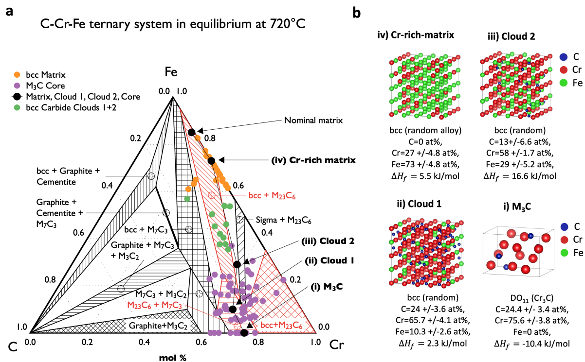
Figure 5. (a) The ternary Fe-Cr-C system at 720 °C with equilibrium data taken from FactSage [50]. The dots indicate data from the chemical profile in Figure 4b, for the M 3 C core and bcc carbide Clouds 1 and 2 used for the DFT calculations in (b).
