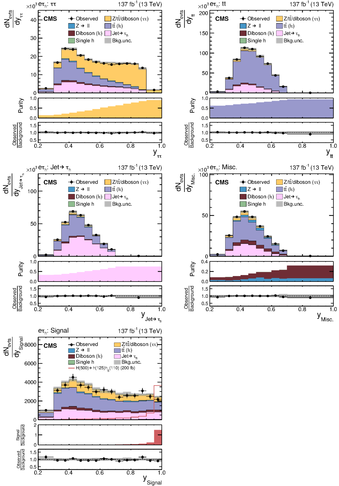
Figure 2: Event categories after NN classification based on a training for m_H = 500 \text{ GeV} and 100 \leq m_{h_s} < 150 \text{ GeV} in the e\tau_h final state. Shown are the (upper left) \tau\tau , (upper right) t\bar{t} , (middle left) \text{jet} \rightarrow \tau_h , (middle right) misc, and (lower left) signal categories. For these figures the data sets of all years have been combined. The uncertainty bands correspond to the combination of statistical and systematic uncertainties after the fit to the signal plus background hypothesis for m_H = 500 \text{ GeV} and m_{h_s} = 110 \text{ GeV} .
