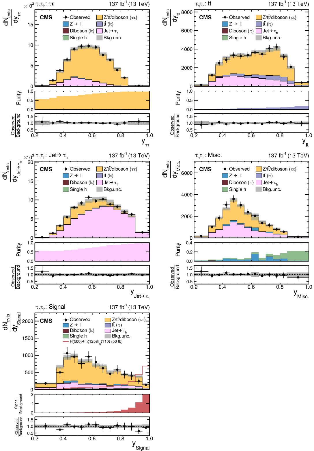
Figure 4: Event categories after NN classification based on a training for m_H = 500 \text{ GeV} and 100 \leq m_{h_s} < 150 \text{ GeV} in the \tau_h \tau_h final state. Shown are the (upper left) \tau\tau , (upper right) t\bar{t} , (middle left) \text{jet} \rightarrow \tau_h , (middle right) \text{misc} , and (lower left) \text{signal} categories. For these figures the data sets of all years have been combined. The uncertainty bands correspond to the combination of statistical and systematic uncertainties after the fit to the signal plus background hypothesis for m_H = 500 \text{ GeV} and m_{h_s} = 110 \text{ GeV} .
