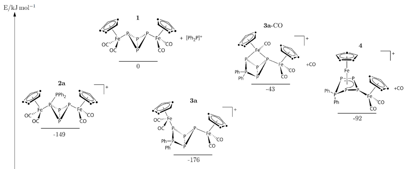
Scheme 3. Relative energies of starting material 1 and [PPh_2]^+ , 3a and its decarbonylation to 4 on the BP86/def2-SVP level.
