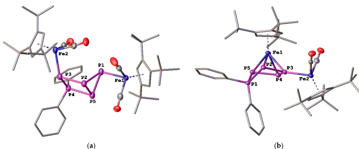
Figure 1. Cationic parts of the molecular structures of 3a (a) and 4 (b), respectively, in the solid state. Hydrogen atoms, solvent molecules and counter ions are omitted for clarity. Selected bond lengths (Å) for 3a —Fe1-P1 2.3162(12), Fe2-P3 2.3004(15), P1-P5 2.2010(18), P2-P1 2.1971(15), P2-P5 2.2546(17), P3-P2 2.2305(15), P3-P4 2.2128(17), P4-P5 2.1974(16). Selected bond lengths (Å) for 4 —Fe1-P3 2.2925(7), Fe1-P5 2.3422(7), Fe1-P4 2.3517(8), Fe1-P2 2.3610(8), Fe2-P3 2.2567(7), P1-P5 2.1590(9), P1-P2 2.1761(9), P2-P3 2.1293(9), P3-P4 2.1337(9), P4-P5 2.1322(10).
