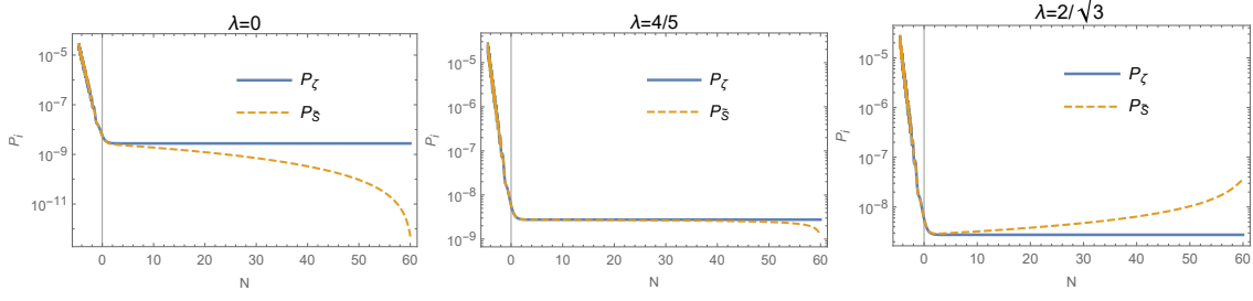
Figure 2. Adiabatic and isocurvature power spectra (in terms of \tilde{S} ) for the system described by (3.23) and (3.24) with m_2 = 0 . Left: for \lambda = 0 the isocurvature perturbations decay on super-horizon scales. Centre: for \lambda = 4/5 the mass of the isocurvature perturbations is tachyonic but the isocurvature power spectrum still decays because of Hubble friction. Right: for \lambda = 2/\sqrt{3} we have tachyonic isocurvature modes that produce an exponential growth of \tilde{S} .
