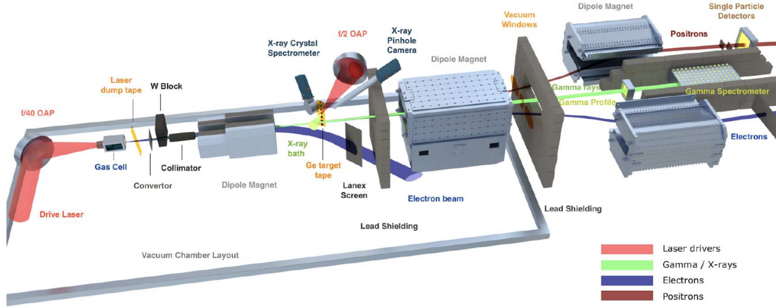
Figure 1. The experiment setup. An f/40 laser pulse was used to drive a laser-wakefield accelerated electron beam in a gas cell. This high-energy electron beam was used to create on axis \gamma -rays before being swept away by a magnet. A second laser pulse was incident on a germanium target tape, driving an x-ray bath through which the \gamma beam passed. Any particle pairs created in this interaction region propagate on axis and are swept away to single particle detectors using a magnetic transport system.
