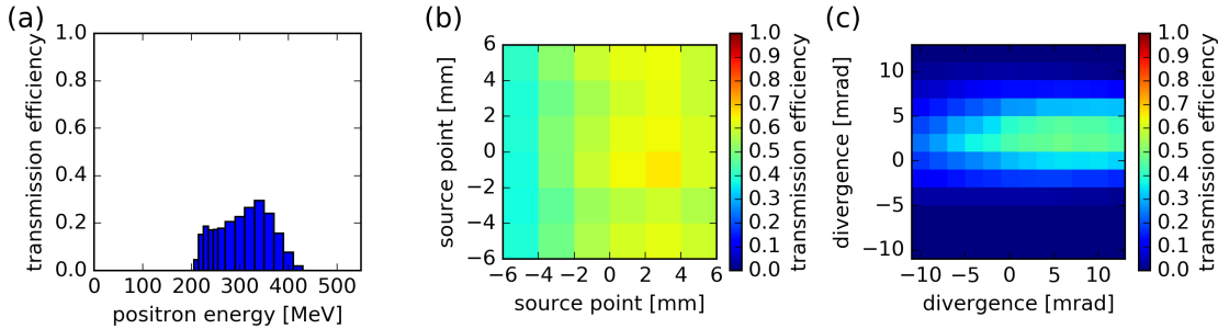
Figure 7. Transmission efficiency of positrons through the AMS to the CsI SPD depending on positron energy (a), source point (b) and divergence (c). For BW positrons, the integrated efficiency is 38% above 200 MeV and 14% overall.
