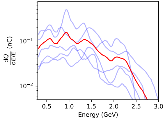
Figure 14. High energy electron beams obtained during a previous Gemini experiment. Taken from ref [53]
