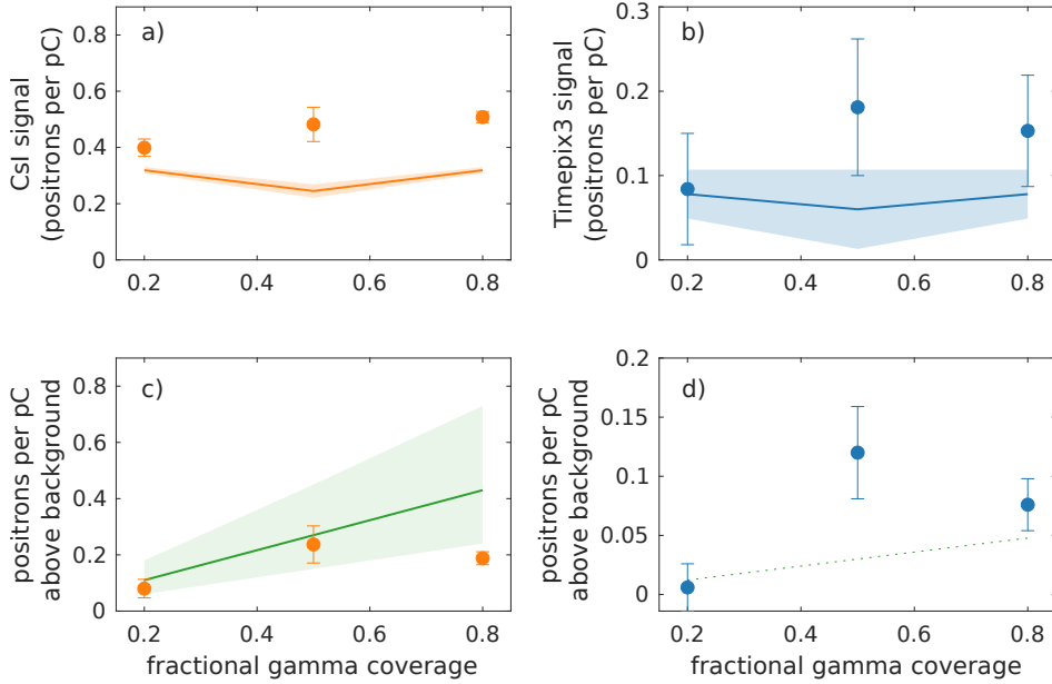
Figure 12. Commissioning of the single particle detectors. Positrons are generated by colliding a fraction of the \gamma beam with a 25 \mu\text{m} thick Kapton target. (a) Positron signal measured (after gamma background subtraction) on the CsI single particle detector. The shaded region is the measured background on a series of shots with the Kapton removed. (b) Positron signal measured on the Timepix3 detector. The shaded region is the measured background on a series of shots with the Kapton removed. (c) Positrons above null shot background measured on the CsI detector. The shaded region is the predicted number of positrons transported to the detector under the same experimental conditions. (d) Positrons above null shot background measured on Timepix3 detector. The dashed line is an estimate of predicted number based on scaling the estimated number of positrons on the larger CsI detector.
