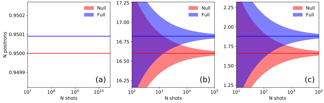
Figure 13. Mean number of positrons and 2\sigma error against number of shots, for both full and null shots. (a) Predictions based on measurements made during the experiment. (b) Predictions based on optimum photon sources and the existing shielding configuration. (c) Predictions based on optimum photon sources, but with an extended setup that reduces the background noise by a factor of ten.
