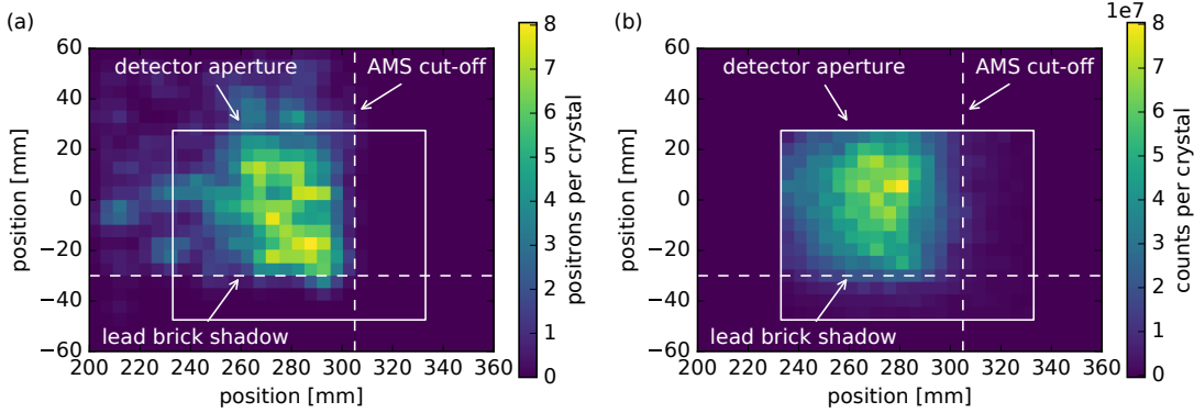
Figure 8. (a) The simulated positron hit map on the detector plane produced by the PTFE calibration target on a 9.2 \text{ pC}_r shot. (b) The measured detector response with the PTFE calibration target in the beam. The combined information from both images is used as a detector calibration.
