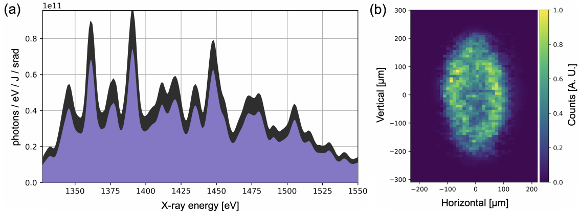
Figure 5. (a) Average x-ray spectra emitted by the germanium target. Measured using a TIAP crystal spectrometer over 47 shots. The standard deviation is given by the black shaded area. (b) Example median-filtered x-ray pinhole camera image of the germanium target. The aspect ratio of the x-ray source closely resembles the f/2 focal spot.
