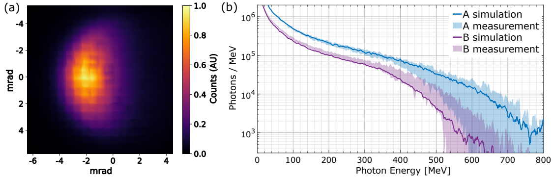
Figure 4. Properties of the \gamma -ray photon source: (a) \gamma beam profile example. The D-shaped footprint produced by the collimator and half-block shadows is clear. (b) Simulated \gamma spectra for both data sets (solid lines) and 1\sigma interval of the first 10 spectra of the corresponding data sets measured with the \gamma spectrometer (shaded regions).
