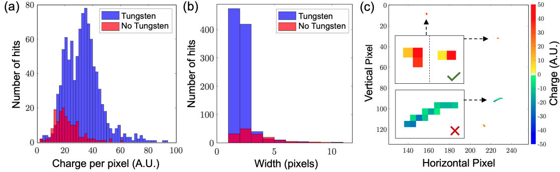
Figure 9. TimePix3 training data. Average charge per pixel (a) and cluster width (b) distributions for shots with and without an on-axis positron source (Tungsten). The difference in the distributions with and without the positron source form the basis of a positron event specification. (c) Examples of the positron specification being implemented and rejecting non-conforming hits (highlighted with a negative colour value).
