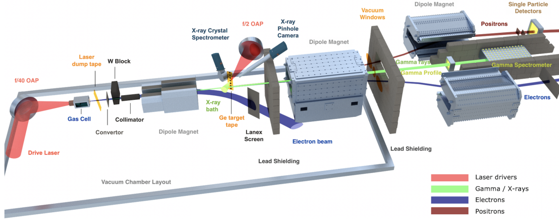
Figure 1. The experiment setup. An f/40 laser pulse was used to drive a laser-wakefield accelerated electron beam in a gas cell. This high-energy electron beam was used to create on axis \gamma -rays before being swept away by a magnet. A second laser pulse was incident on a germanium target tape, driving an x-ray bath through which the \gamma beam passed. Any particle pairs created in this interaction region propagate on axis and are swept away to single particle detectors using a magnetic transport system.
