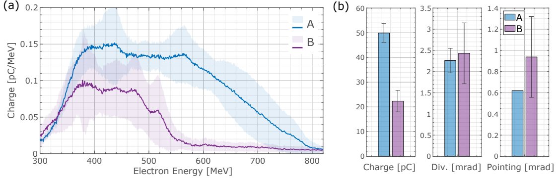
Figure 3. Properties of the electron beam used to generate the \gamma -ray photon source: (a) Average electron spectra with standard deviation from mean (shaded). (b) Average electron beam properties with standard deviations (error bars). A (blue) and B (purple) represent the optimum beam performance and performance during commissioning, respectively.
