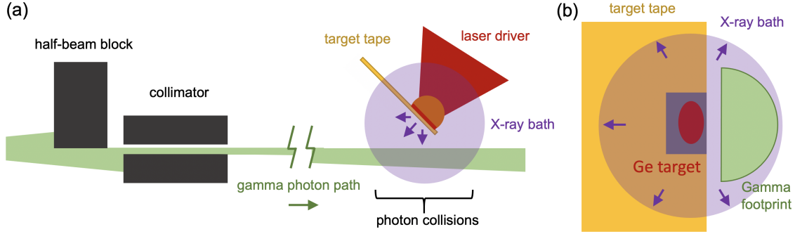
Figure 2. (a) Simplified view of the photon collision geometry. The tungsten half-beam block and collimator shape the \gamma beam to the desired profile before, much further downstream, colliding with the pre-expanded x-ray bath. (b) On-axis view of the overlap geometry. The x-ray bath radiates in all directions from the germanium target dot, providing a suitable particle-free collision volume for the D-shaped \gamma beam to pass through.
