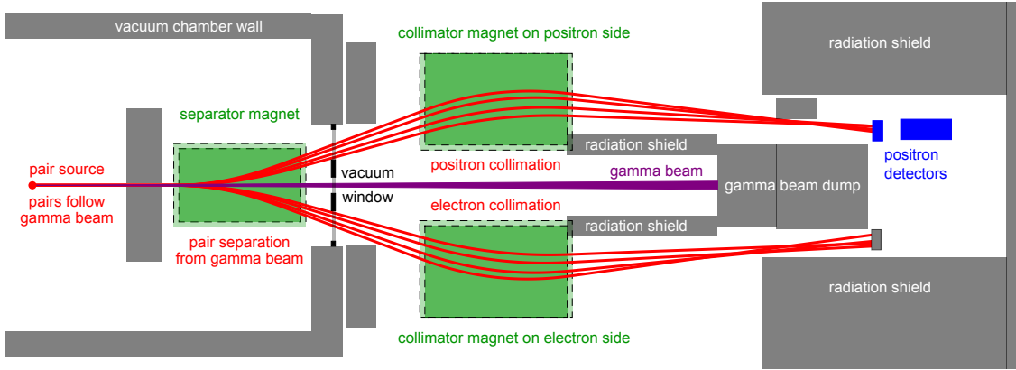
Figure 6. Overview of the analyser magnet system (AMS) to transport generated pairs to the single particle detectors (SPD). The combination of separator and collimator magnets was adapted for the energy range in this experiment by adjusting the length of the magnets and their separation. The electron and positron paths were adjusted to avoid the SPDs being directly exposed to radiation from noise sources inside the vacuum chamber (such as the electron source and converter target).
