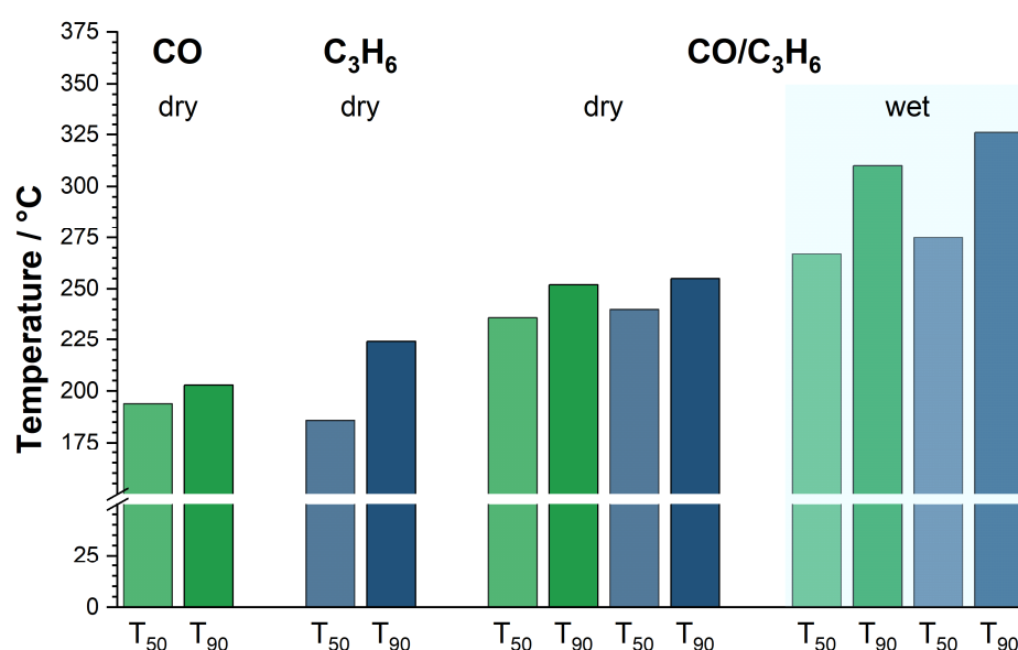
Figure 2. Temperatures of 50% (lighter shades) and 90% (darker shades) conversion for CO (green), C 3 H 6 (blue) and CO/C 3 H 6 oxidation reactions catalyzed by Pt single site.
