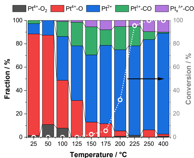
Figure 6. Fraction of the different Pt species at the middle of the catalyst bed, as determined by MCR-ALS and conversion of CO (empty circles connected via dotted line) as function of temperature in reaction mixture (1000 ppm CO, 10% O 2 in He).
