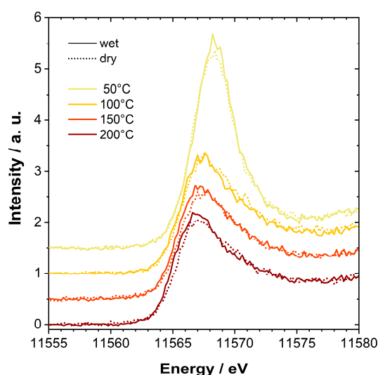
Figure 7. HERFD-XANES spectra recorded during CO temperature programmed reduction (1000 ppp Co/He), in absence (dotted lines) or presence (solid lines) of water in the gas feed ( H_2O < 6\% ).
