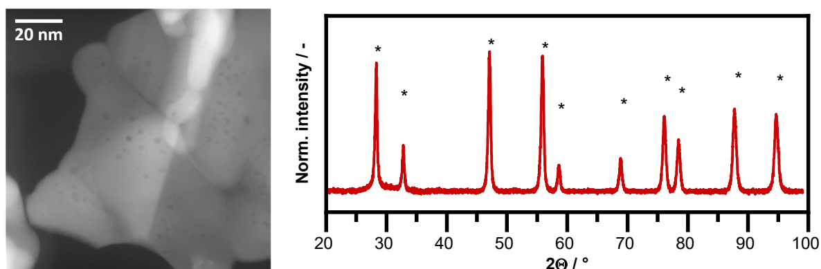
Figure 1. TEM micrograph of Pt-single site samples evidence the absence of Pt nanoparticles (left); XRD diffractogram of the sample (right). Stars indicate the reflections typical for CeO 2 .
