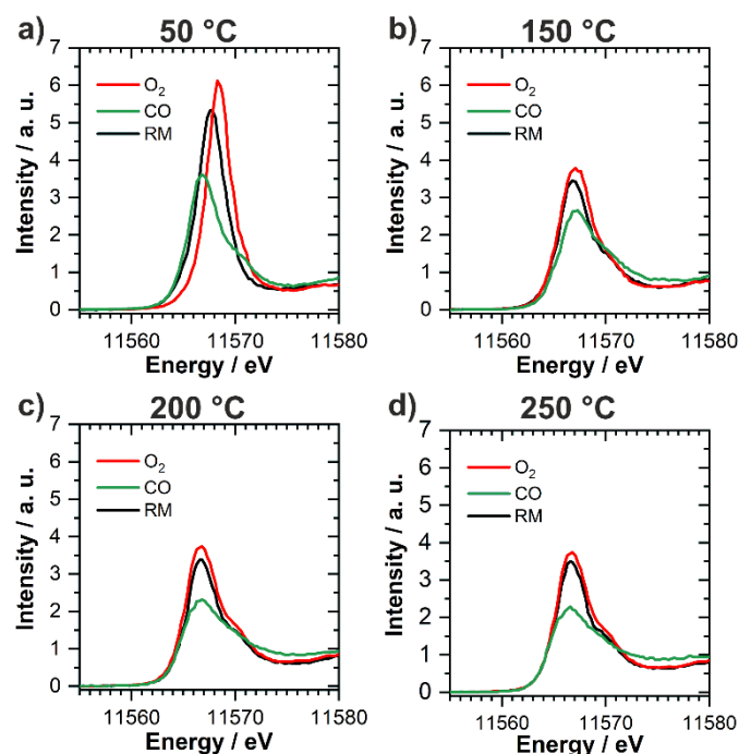
Figure 4. (a–d) Evolution with temperature of HERFD-XANES spectra of Pt single sites on CeO 2 under different gas atmospheres, as collected at the middle position of the catalyst bed (red curves: 10% O 2 /He, green curves: 1000 ppm CO/He and black curves: reaction mixture with 1000 ppm CO, 10% O 2 in He).
