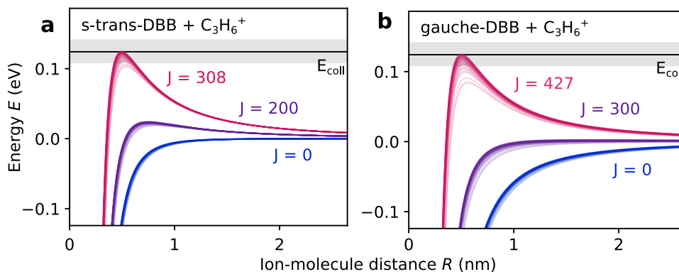
Figure 5: Rotationally adiabatic, centrifugally corrected ion-molecule interaction potentials for the reaction of a s-trans - and b gauche -DBB with propene ions for different values of the total collisional angular momentum quantum number J . Each value of J comprises a set of lines corresponding to all rotational states of DBB with rotational angular momentum quantum number j = 4 which corresponds to the largest population in the molecular beam. The collision energy E_{\text{coll}} is indicated by the black horizontal line and the grey-shaded areas represent its experimental uncertainty.
