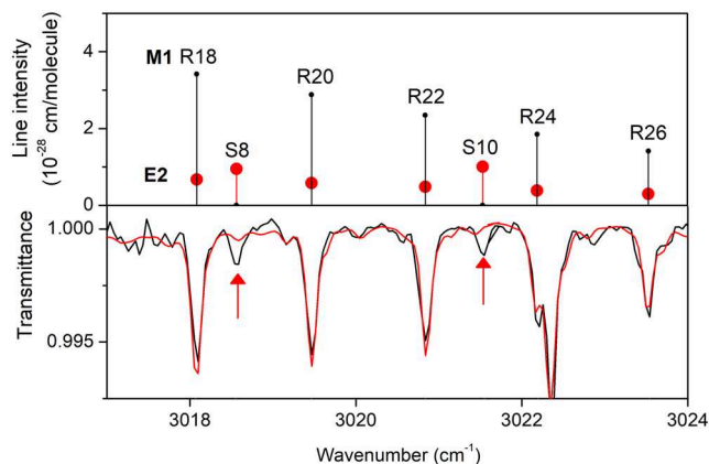
FIG. 2. Comparison of the ACS MIR transmission spectra of the atmosphere of Mars 21 near 3020 cm -1 with the calculated line lists of the M1 and E2 \nu_2 + \nu_3 bands of ^{12}\text{C}^{16}\text{O}_2 . Upper panel: The presently calculated E2 transitions with ab initio intensities (red stems) are superimposed to the M1 transitions with intensities calculated in Ref. 61 (black stems). Lower panel: The ACS MIR spectrum (red line) with a best-fit synthetic model containing the contributions of the E1 bands of \text{CO}_2 and \text{H}_2\text{O} based on the HITRAN 2016 database and of the M1 lines identified in Ref. 21. The assignments of the newly detected S8 and S10 E2 transitions are marked with red arrows.
