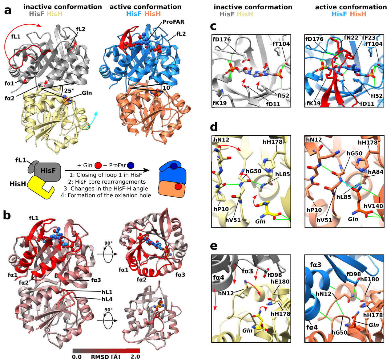
Fig. 2 Structural changes in the HisFH complex upon allosteric activation. a Crystal structure of the HisFH complex (hC84A) in the inactive conformation (HisF in gray, HisH in yellow; PDBID: 7AC8, chains C/D) bound to Gln (left) and in the active conformation (HisF in marine, HisH in orange, chains E/F) bound to ProFAR and Gln (right). The largest structural differences between the two conformations are observed in HisF (red arrows). The reorientation of HisH relative to HisF is indicated by a cyan arrow and leads to a reduction of the angle between ff120, hw123 and hG52 (C \alpha atoms) from 25° to 10°. The major structural changes between the inactive and active conformations are indicated as cartoons. b The local backbone RMSD between the inactive and active conformations (PDBID 7AC8, chains C/D and E/F), after individual alignment of the proteins, mapped onto the structure of the active conformation. c Closeup of the HisF active site: Comparison between the inactive (left; PDBID 7AC8; chain A) and the active conformation (right; PDBID 7AC8, chain E). Important hydrogen bond interactions are shown in green. fl1 is shown in red. The compaction of the HisF active site in the active conformation is indicated by red arrows. d Oxyanion hole formation in the active conformation of HisH: The oxyanion hole is not formed in the inactive conformation (left; PDBID 7AC8, chain D). Red arrows indicate important conformational changes upon formation of the active conformation. The oxyanion hole (right; PDBID 7AC8, chain F) is formed by the rotation of the hG50/hV51 amide group. The side chain of the substrate Gln rotates into the oxyanion hole and forms hydrogen bonds to hG50 and hL85 (cyan). Other hydrogen bonds are shown in green. e The rearrangement of the HisF–HisH interface moves fa3/α4 and fd98 closer to the active site (red arrows). Upon transition from the inactive (left; PDBID 7AC8, chains C/D) into the active conformation (right; PDBID 7AC8, chains E/F) fd98 moves by 3.6 Å and interacts with hn12. Additional backbone hydrogen bonds are formed that connect hL4 and hα1 in HisH with fa4 and α3 in HisF.
