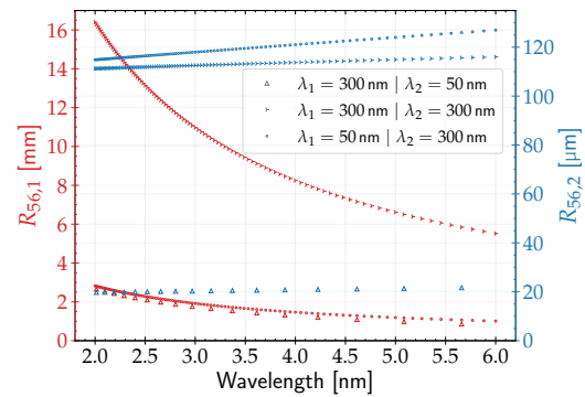
(b) Optimum setup of the chicanes to maximize the bunching factor. The working point resulting in a lower R_{56,1} is shown for each configuration.
