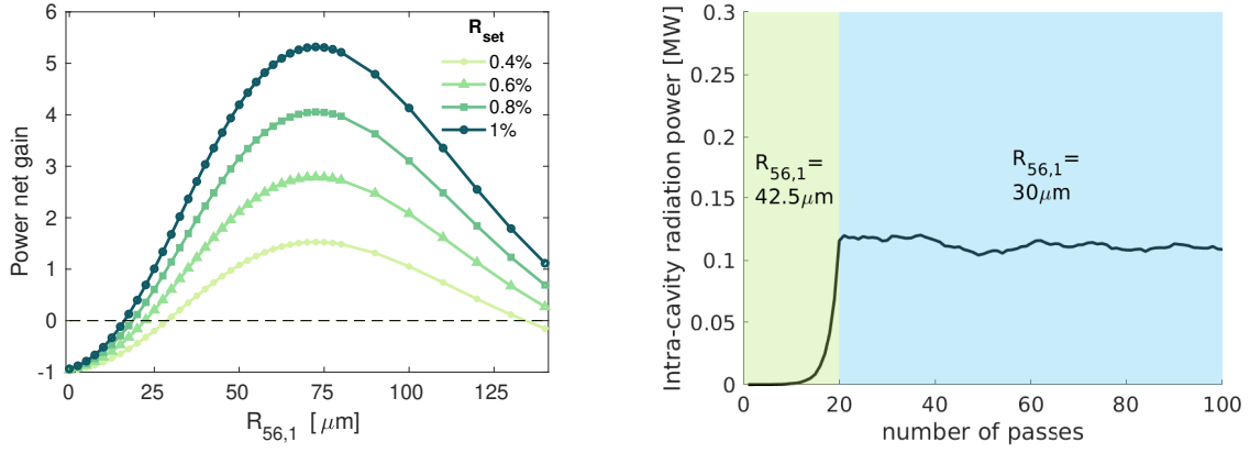
(a) Changing the R_{56,1} of the chicane affects drastically the gain in power. Here we show the net power gain for selected set reflectivities R_{\text{set}} , between 0.4% and 1%. The horizontal line shows the zero net gain.
