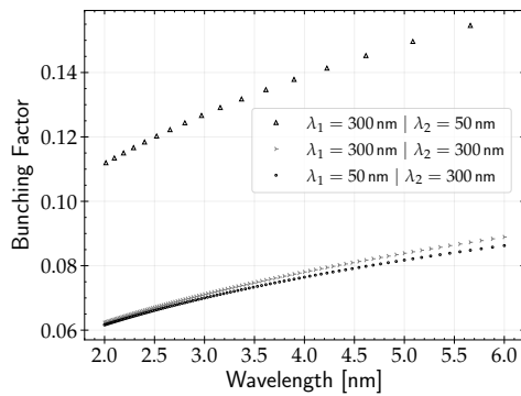
(a) Maximum bunching factor for different combinations of seed laser wavelengths.
