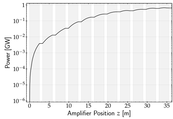
(b) FEL peak power along the amplifier modules (gray).
