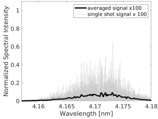
(a) SASE. Please notice the extended horizontal axis. The average SASE spectrum over 50 shots is shown with the black line.
