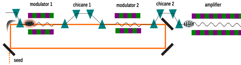
Figure 9. In an oscillator-based HGHG scheme, an optical klystron can be employed. To do so, the cavity contains two modulators separated by a chicane. This way this chicane can be tuned to control the gain per pass.
