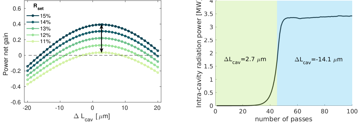
(a) Detuning curves for a 300 fs flat-top electron beam. The optimum detuning length is at \Delta\lambda = 2.7 \mu\text{m} , for all set reflectivities, as shown with the vertical arrow. The zero net gain point shown with the horizontal dashed line, shows the detuning that needs to be applied to reach equilibrium for each total reflectivity R_{set} . Keeping the reflectivity constant and changing the cavity length can transition the system from positive to zero net gain.
