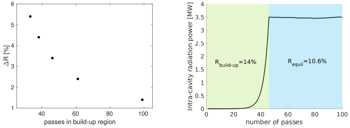
(a) In this plot, the number of passes needed to reach steady-state as function of reflectivity change, \Delta R = R_{\text{build-up}} - R_{\text{equil}} , is shown. We assume that the build-up process is over when the energy modulation is at least A=7 .
