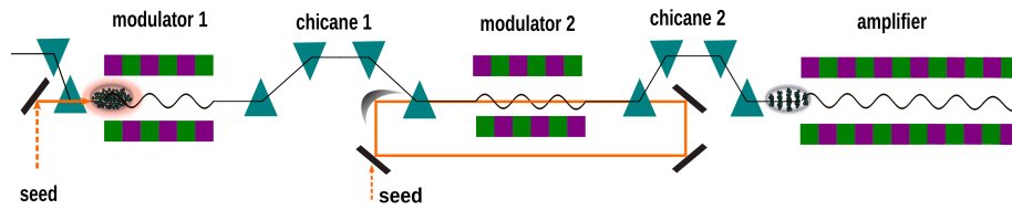
Figure 3. In an oscillator-based EEHG scheme, one or two optical cavities can be attached. In this figure, the first modulation occurs with a conventional external seed laser, while the second energy modulation is achieved by employing an optical cavity around the second modulator. The optical cavity is fed by a seed laser and maintains its properties in order to seed consecutive electron bunches.
