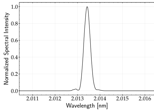
(c) Spectrum after the 5 modules of the amplifier.
