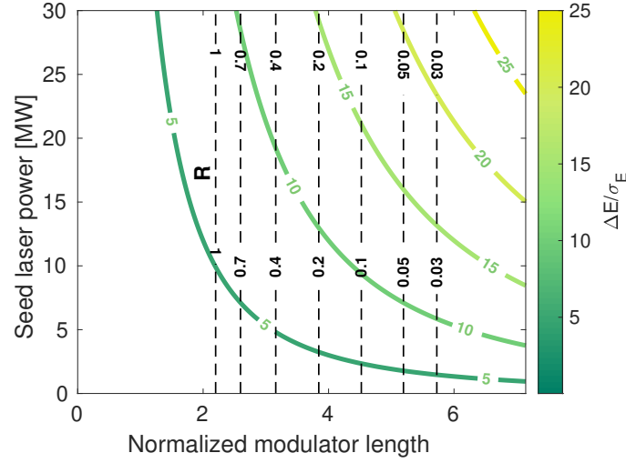
Figure 6. The colorbar indicates the energy modulation achieved for combinations of seed laser powers ( P_{in} ) and modulator lengths ( L_{mod} ) and is calculated with Eq. 3. The horizontal axis shows the normalized modulator length to the gain length ( L_{mod}/L_g ). The vertical dashed lines show the reflectivity R required for equilibrium between amplification and losses for different normalized modulator lengths, and is calculated with Eq. 2.
