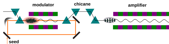
Figure 1. In an oscillator-based HGHG scheme, an optical cavity is added and encloses the modulator. The optical cavity acts as a feedback system which maintains the power level of the stored radiation field and, under perfect synchronism, this field is used to seed consecutive electron bunches arriving from the linac upstream the cavity. It should be noted that in reality, the optical cavity design will be more complex than this simplified sketch.
