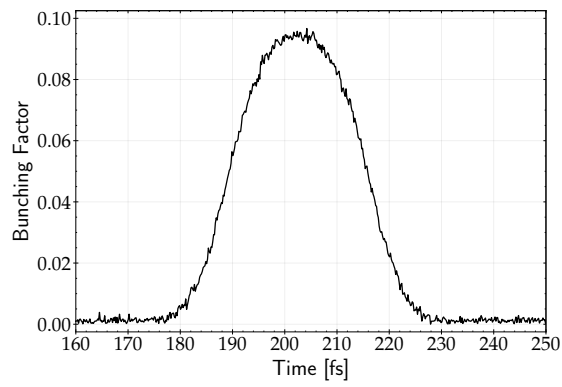
(a) Bunching along the electron bunch.
