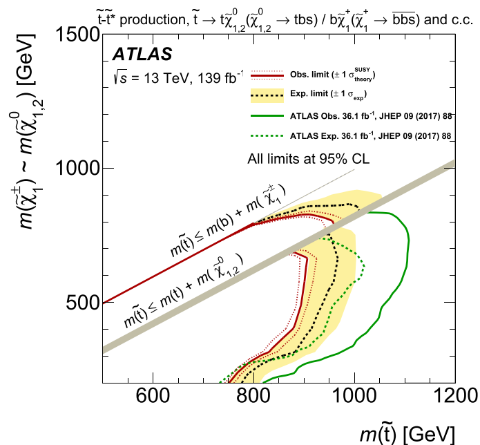
Fig. 8 Observed and expected exclusion contours for the \tilde{t} and \chi_1^\pm masses in a top-squark production model with RPV decays of the \chi_1^\pm and of the \tilde{\chi}_{1,2}^0 . Limits are shown in the case of a higgsino LSP. The contours of the band around the expected limit are the \pm 1\sigma variations, including all uncertainties except theoretical uncertainties in the signal cross-section. The dotted lines around the observed limit illustrate
