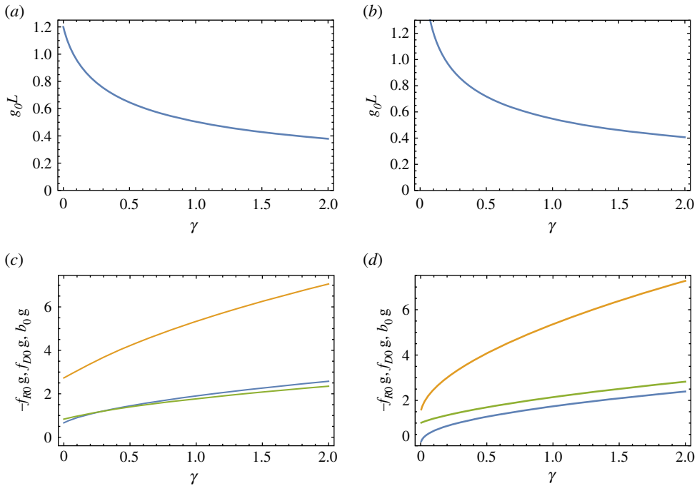
Figure 4. Dependence of the TRL lens parameter g_0L on the relative gap of the lenses \gamma for the apochromatic condition of (a) Type I and (b) Type II lens system. The corresponding focal lengths and image distances of -f_{R0} (blue), f_{D0} (green) and b_0 (orange) in the apochromatic condition, in units of 1/g for (c) Type I and (d) Type II lens system. (Online version in colour.)
