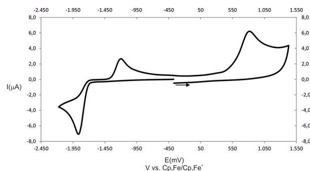
Figure 3. Cyclic voltammogram of 1b in \text{CH}_2\text{Cl}_2/n\text{Bu}_4\text{NPF}_6 solution at r.t. and \nu = 0.1 V s −1 .
