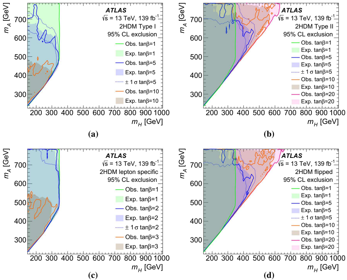
Fig. 10 Observed and expected 95% CL exclusion regions for the \ell\ell b\bar{b} channel in the (m_H, m_A) plane for various \tan\beta values for the a type-I, b type-II, c lepton-specific and d flipped 2HDM, with \cos(\beta - \alpha) = 0
