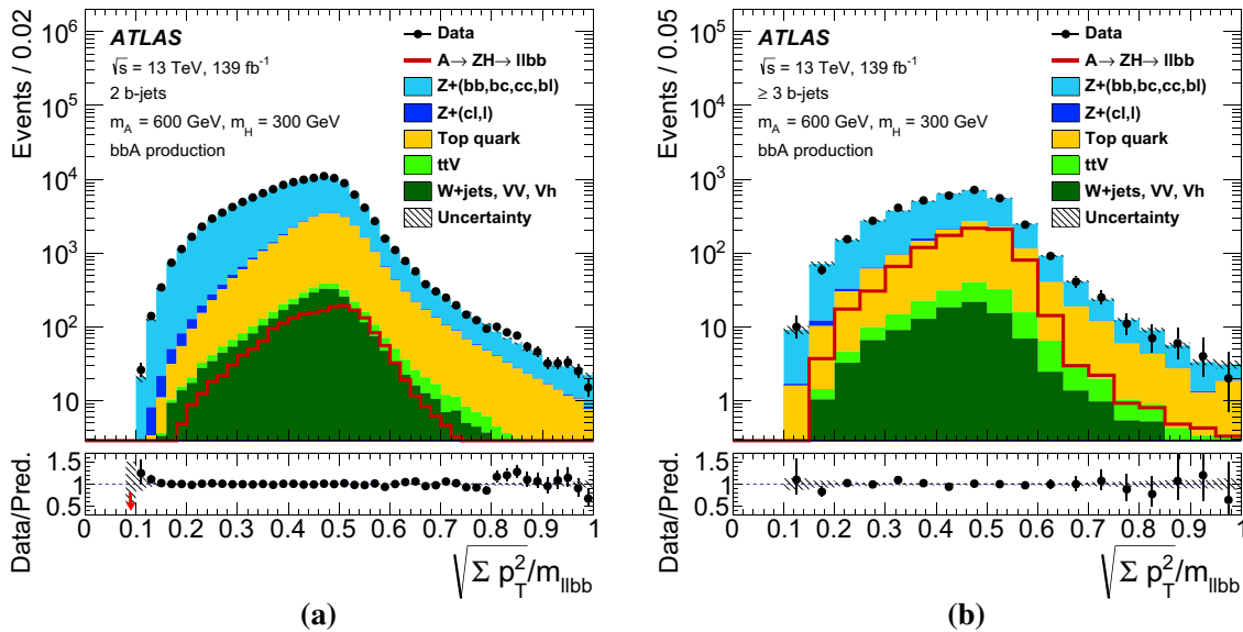
Fig. 2 The \sqrt{\sum p_T^2 / m_{\ell\ell bb}} distributions shown before the requirement on this variable is applied for events with a exactly two b -jets and b three or more b -jets. Corrections from a fit to the data are applied to the simulation, as described in Sects. 5.1 and 8. The signal distribution for (m_A, m_H) = (600, 300) GeV is also shown, and is normalised such that the production cross section times the branching ratios B(A \rightarrow ZH) and B(H \rightarrow bb) corresponds to 1 pb. The signal shown includes only A bosons produced in association with b -quarks. The lower panel shows the ratio of the data to the background prediction (black filled circles) and the relative uncertainty,
