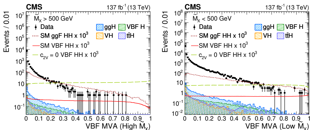
Figure 6. The distribution of the two MVA outputs is shown in data and simulated events in the two VBF \widetilde{M}_X regions: \widetilde{M}_X > 500 GeV (left) and \widetilde{M}_X < 500 GeV (right). Data, dominated by the \gamma\gamma +jets and \gamma +jets backgrounds, are compared to the VBF HH signal samples with SM couplings and c_{2V} = 0 , SM ggF HH and single H samples ( t\bar{t}H , ggH, VBF H, VH) after imposing the VBF selection criteria described in section 5. The error bars on the data points indicate statistical uncertainties. The HH signal has been scaled by a factor of 10^3 for display purposes.
