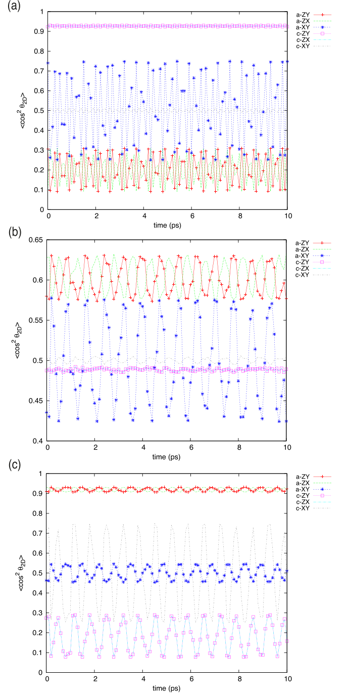
FIG. 9. Calculated 2D alignment-cosine time-profiles for wave packets generated with an optical centrifuge with field strength E_0 = 2 \times 10^8 V/cm and three different acceleration rates [(a)–(c)] \beta = 30 , 115, and 230 GHz/ps, respectively. The centrifuge-field release times were 228, 133, and 66 ps, respectively, see Fig. 4. The alignment cosines measure the degree of alignment of the principal axes of inertia of D 2 S with respect to the laboratory axes defined by the centrifuge field. For instance, a - ZY is the 2D alignment cosine calculated with respect to the laboratory Z axis of the projection of the molecular a axis onto the ZY detector plane.
