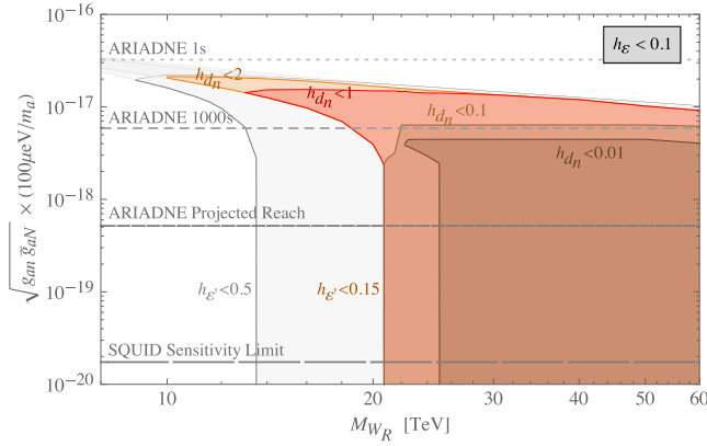
FIG. 1. Regions in the LR DFSZ model of the CPV axion nucleon coupling probed by ARIADNE.
