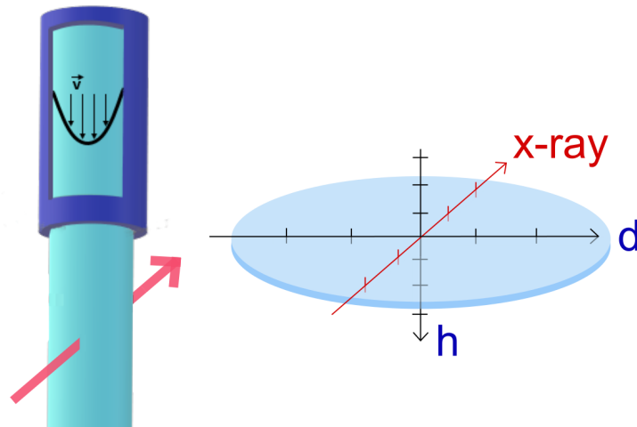
Figure 5.1: Sketch of a Rayleigh nozzle. The X-ray beam hits the jet perpendicular to the flow direction with h = 0 at the nozzle tip. The center of the jet is defined as d = 0 with d > 0 denoting the right-hand side of the jet with respect to the incoming X-ray beam.
