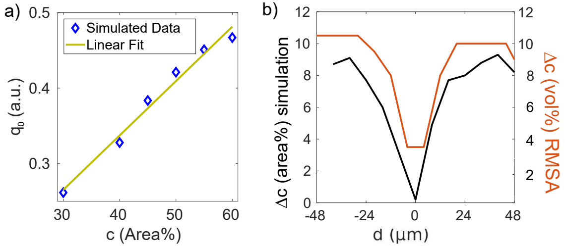
Figure 7.6: a) The position of q_0 for different area concentrations is shown for simulated 2-dimensional diffraction patterns. b) Concentration difference \Delta c across the jet approximated by q_0 positions. The slope of the linear fit in a) was extracted to convert measured q_0 variances in \varphi into concentration differences. Additionally the concentration difference calculated using the RMSA from Fig. 5.9 b is shown.
