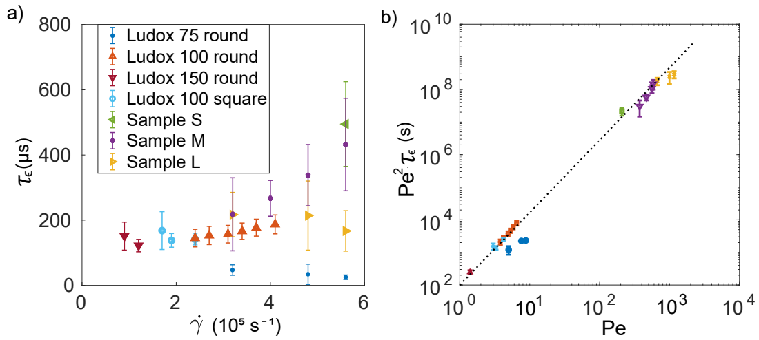
Figure 5.12: a) The characteristic decay time \tau_\epsilon from the exponential fit of \xi_\epsilon for Ludox ( r = 15 \text{ nm} ) and samples S ( r = 43 \text{ nm} ), M ( r = 63 \text{ nm} ) and L ( r = 77 \text{ nm} ). Data for the Ludox sample was taken with 75\mu\text{m} (blue), 100\mu\text{m} (orange) and 150\mu\text{m} (red) round tubes as well as the 100\mu\text{m} square tube (light blue). b) Characteristic times \tau_\epsilon (see Tab.5.1 and Tab.5.2) were weighted with the square of the Péclet number Pe^2 and are shown as a function of Pe . The data points collapse on a straight line.
