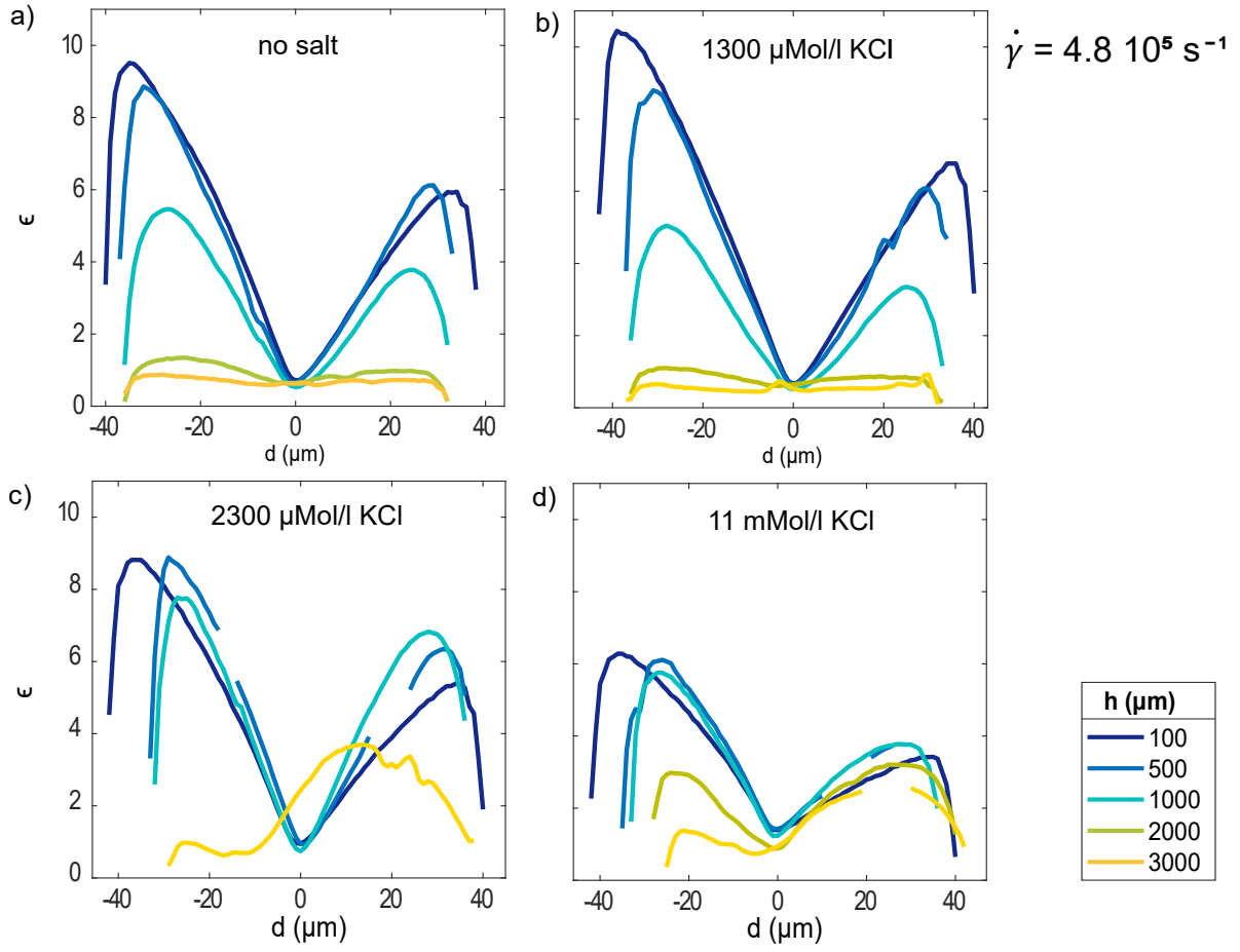
Figure A3: Plotted is the asymmetry quantifying parameter \epsilon over the nozzle profile d for sample L with a) no salt, b) 1300 \mu\text{Mol/l} , c) 2300 \mu\text{Mol/l} and d) 11 mMol/ KCl. Measurements were performed with the 75 \mu\text{m} round nozzle at \dot{\gamma} = 4.8 \cdot 10^5 \text{ s}^{-1} .
