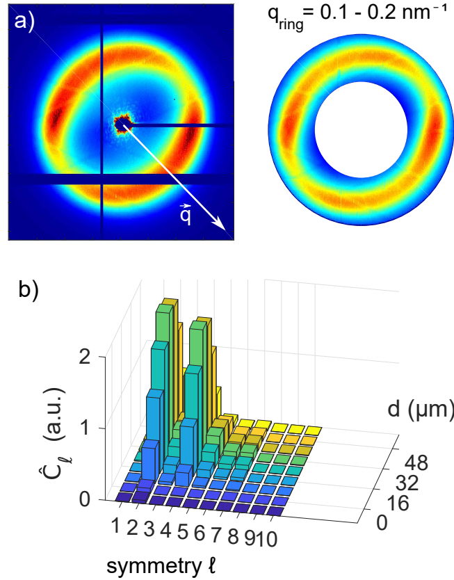
Figure 5.5: a) Diffraction patterns of the Ludox sample and \Delta q cut containing the first intensity maximum between q = 0.1\text{-}0.2 \text{ nm}^{-1} . Gaps between detector panels (dark stripes) have been filled with intensities obtained from mirrored pixels. b) The Fourier coefficients \hat{C}_\ell from XCCA for symmetries \ell = 1\text{-}10 are shown for d > 0 of the same jet described in Fig. 5.4.
