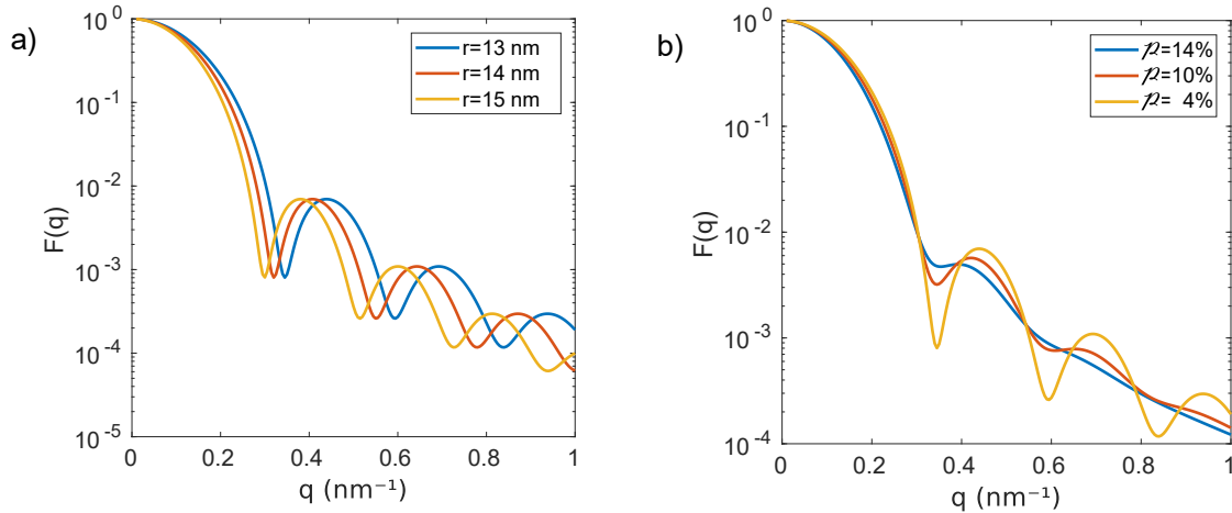
Figure 3.2: Form factor F(q) for a) different particle sizes r at \mathcal{P} = 4\% and b) high and low dispersities \mathcal{P} = \sqrt{\frac{1}{z+1}} (cf. equation 3.10) for particles r = 13 nm.
