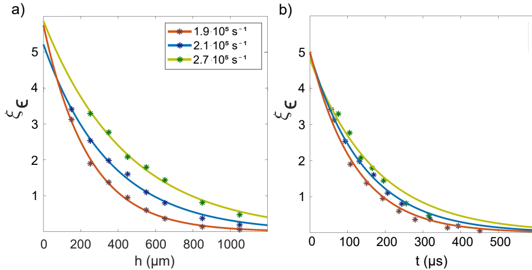
Figure 5.10: a) The maximum of the intensity asymmetry \xi_\varepsilon for Ludox as a function of the distance h from the nozzle tip. Shown are the results for three different shear rates \dot{\gamma} measured with the 100 \mu\text{m} square jet. b) Decay \xi_\varepsilon over time t for the same three data sets as in a).
