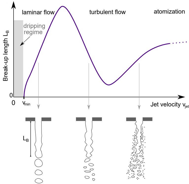
Figure 2.8: Laminar and turbulent jetting regime are distinguished by the break-up length and jet speed (adapted from reference [70]).
