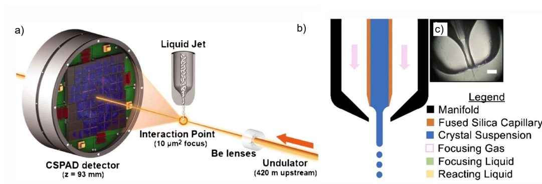
Figure 2.10: a) Application of a liquid jet sample environment for serial femtosecond crystallography (SFX) at an XFEL (CXI instrument, LCLS) 73,74 . b) Schematic for the jet generation from a GDNV and c) photography of an GDNV (adapted from reference [75]).
