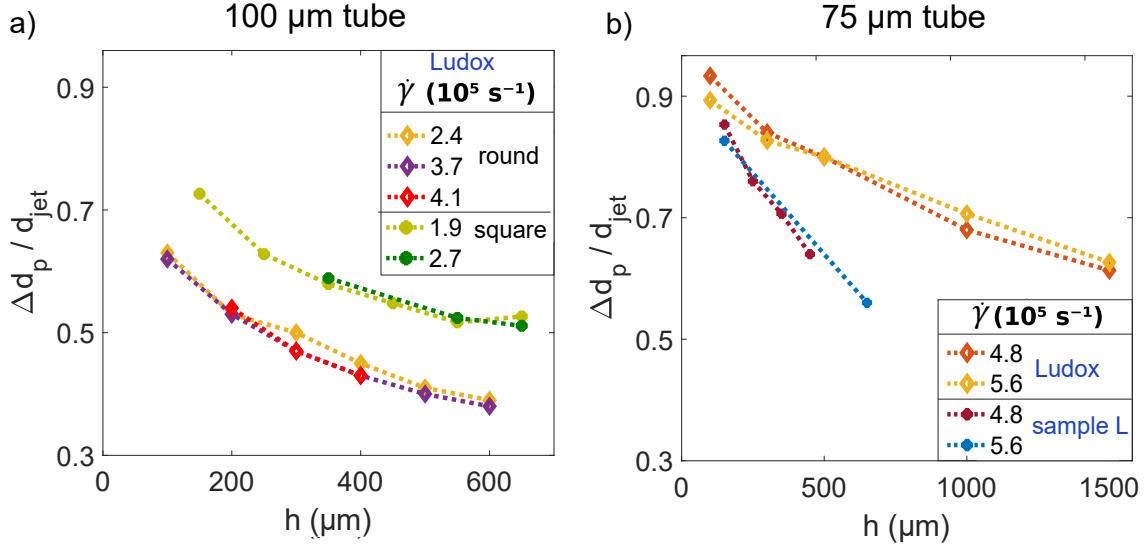
Figure 5.8: a) Distance \Delta d_p between maxima of \varepsilon(d) normalized on the jet diameter d_{jet} as a function of h for a round and a square tube (100 \mu m jet). b) \Delta d_p / d_{jet} over h is shown for the Ludox sample and sample L (75 \mu m jet).
