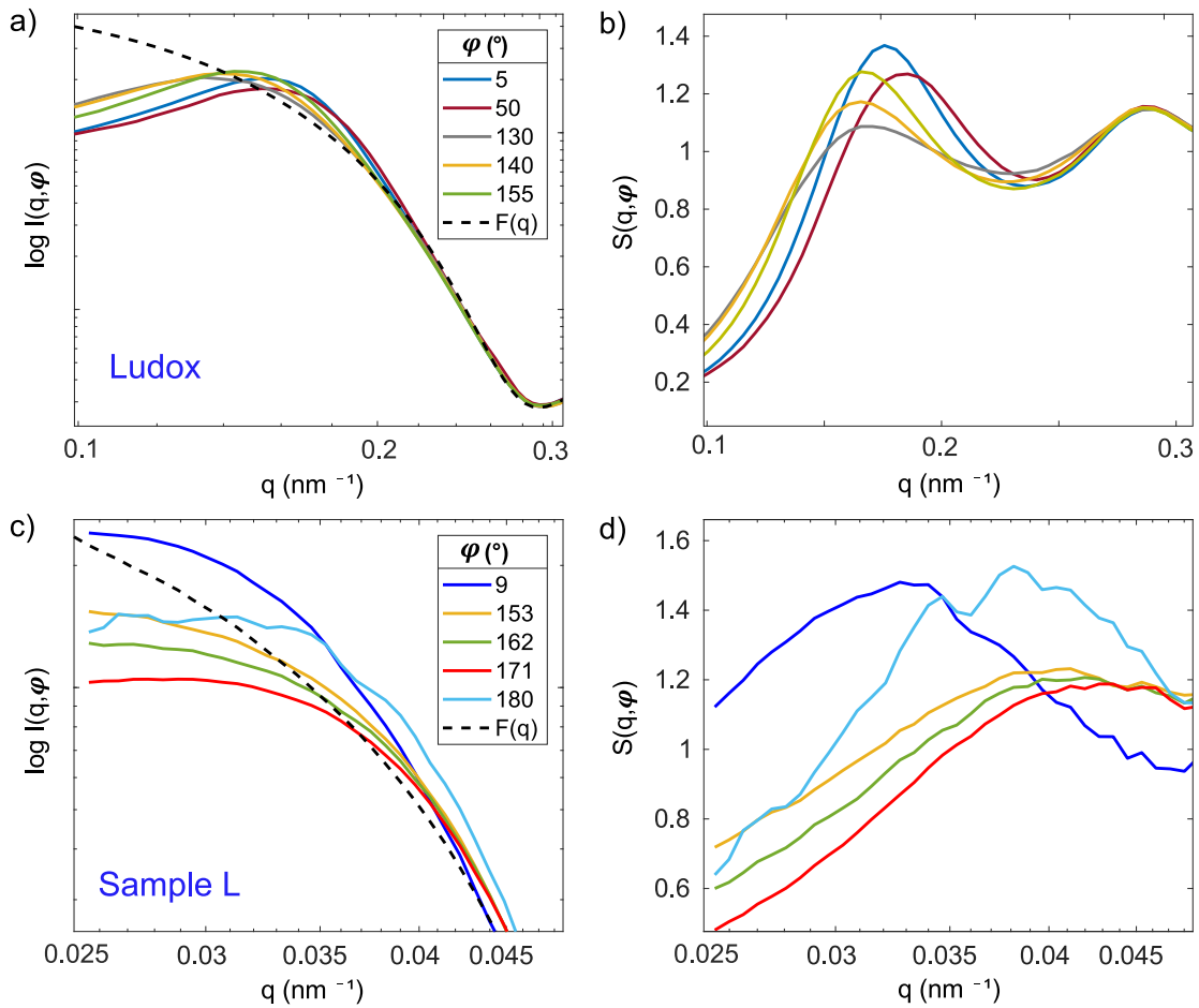
Figure 5.4: a) Intensity I(q, \varphi) of the Ludox sample integrated over circular sectors of \Delta\varphi = 5^\circ and b) structure factors calculated from the intensities shown in a). The measurements were performed at d = 24\mu\text{m} with the 100\mu\text{m} square nozzle, flow rate Q = 1600\mu\text{l}/\text{min} at h = 250\text{mm} nozzle distance. c) Intensity I(q, \varphi) of sample L integrated over circular sectors of 9^\circ and d) structure factors calculated from the intensities shown in c). The measurements were performed at d = 24\mu\text{m} with the 75\mu\text{m} round nozzle, flow rate Q = 800\mu\text{l}/\text{min} at h = 100\text{mm} nozzle distance.
