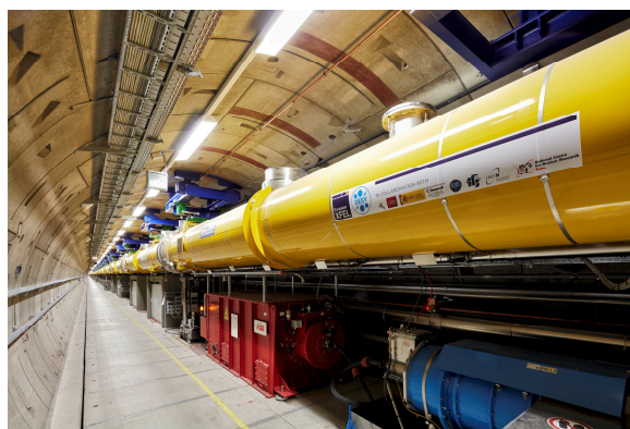
Figure I.4: The European XFEL generates ultrashort (< 100 fs) X-ray flashes – 27 000 times per second with a brilliance that is a billion times higher than that of the best storage ring X-ray sources.
