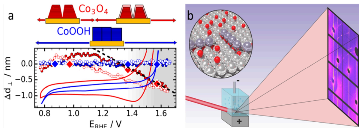
Figure III.3.3: Studying water–electrode interactions: (a) Formation of a nanoscale skin layer on Co 3 O 4 (111) electrodes during OER (0.1 KOH, potential sweep; symbols = layer thickness, lines = electrochemical current). The CoOOH(001) electrode does structurally not change. Reprinted with permission from [3.67]. Copyright 2019 American Chemical Society. (b) Studying atomic-scale mechanisms with high-energy surface X-ray diffraction of Pt surface oxidation with their structural arrangements (upper left).
