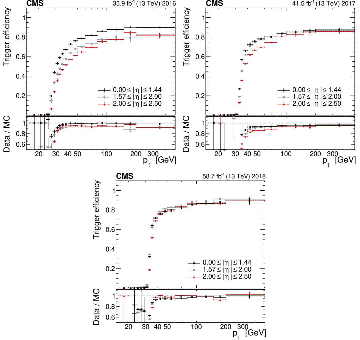
Figure 8: Efficiency of the lowest unprescaled single-electron HLT path (HLT_Ele27_WPTight_Gsf in 2016, HLT_Ele32_WPTight_Gsf in 2017–2018), with respect to the offline reconstruction, as a function of the electron p_T , for different \eta regions using the 2016 (upper left), 2017 (upper right) and 2018 (lower) data sets. The bottom panel shows the data-to-simulation ratio. The efficiency measurements combine the effects of the L1 and HLT triggers. The vertical bars on the markers represent combined statistical and systematic uncertainties.
