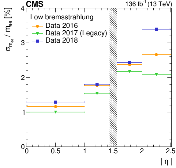
Figure 33: The relative Z mass resolution from Z \rightarrow ee decays in bins of \eta for the barrel and endcaps. Electrons from Z \rightarrow ee decays are used and the resolution is shown for low-bremsstrahlung electrons. The plot compares the resolution achieved for the data collected at 13 TeV during Run 2 in 2016, 2017, and 2018. The 2016 and 2018 data are reconstructed with an initial calibration whereas the 2017 data are reconstructed with refined calibrations. The resolution is estimated after all the corrections are applied, as described in Section 6.3.1, including the scale and spreading corrections of Section 6.2. The grey vertical band represents the region 1.44 < |\eta| < 1.57 and it is not included since it corresponds to the transition between barrel and endcap electromagnetic calorimeters.
