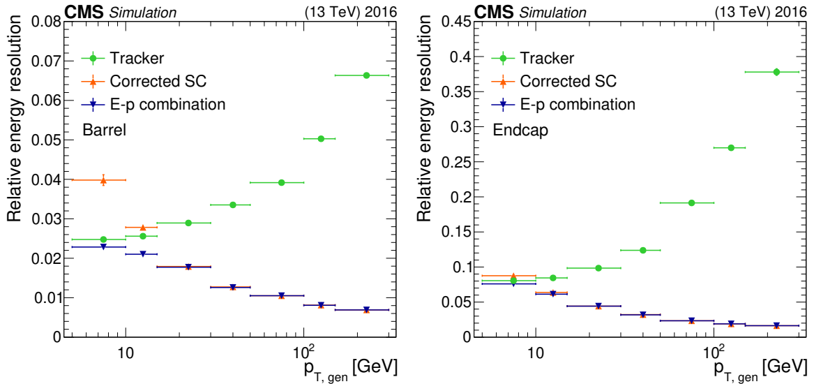
Figure 11: Relative electron resolution versus electron p_T , as measured by the ECAL (“corrected SC”), by the tracker, and seen in the E - p combination, as found in 2016 MC samples for barrel (left) and endcap (right) electrons. Vertical bars on the markers represent the uncertainties coming from the fit procedure.
