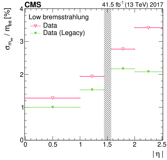
Figure 28: Dielectron mass resolution from Z \rightarrow ee events as a function of the \eta of the electron for the Legacy calibration (green filled markers) and the EOY calibration (pink empty markers) of the 2017 data set. The grey vertical band represents the region 1.44 < |\eta| < 1.57 and it is not included since it corresponds to the transition between barrel and endcap electromagnetic calorimeters.
