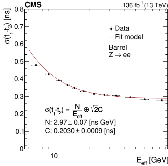
Figure 35: ECAL timing resolution as a function of the effective energy of the electron pairs as measured in 2016, 2017 (Legacy), and 2018 data. Vertical bars on the markers represent the uncertainties coming from the fit procedure used to determine the \sigma(t_1 - t_2) parameters.
