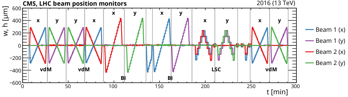
Figure 3: Relative change in the positions of beams 1 and 2 measured by the DOROS BPMs during fill 4954 in the horizontal ( x ) or vertical ( y ) directions, as a function of the time elapsed from the beginning of the program. The gray vertical lines delineate vdM, BI, or LSC scans.
