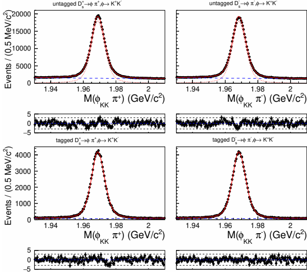
FIG. 3. (color online) Data and fit projection for the reference mode D_s^+ \rightarrow \phi \pi^+ . Left side shows D_s^+ candidates, right side shows D_s^- candidates. Top row is the untagged sample, bottom row is the tagged sample. The red solid line is the total fit, the red dotted line is signal, and the dashed blue line is background. The plots beneath the distributions show the residuals.
