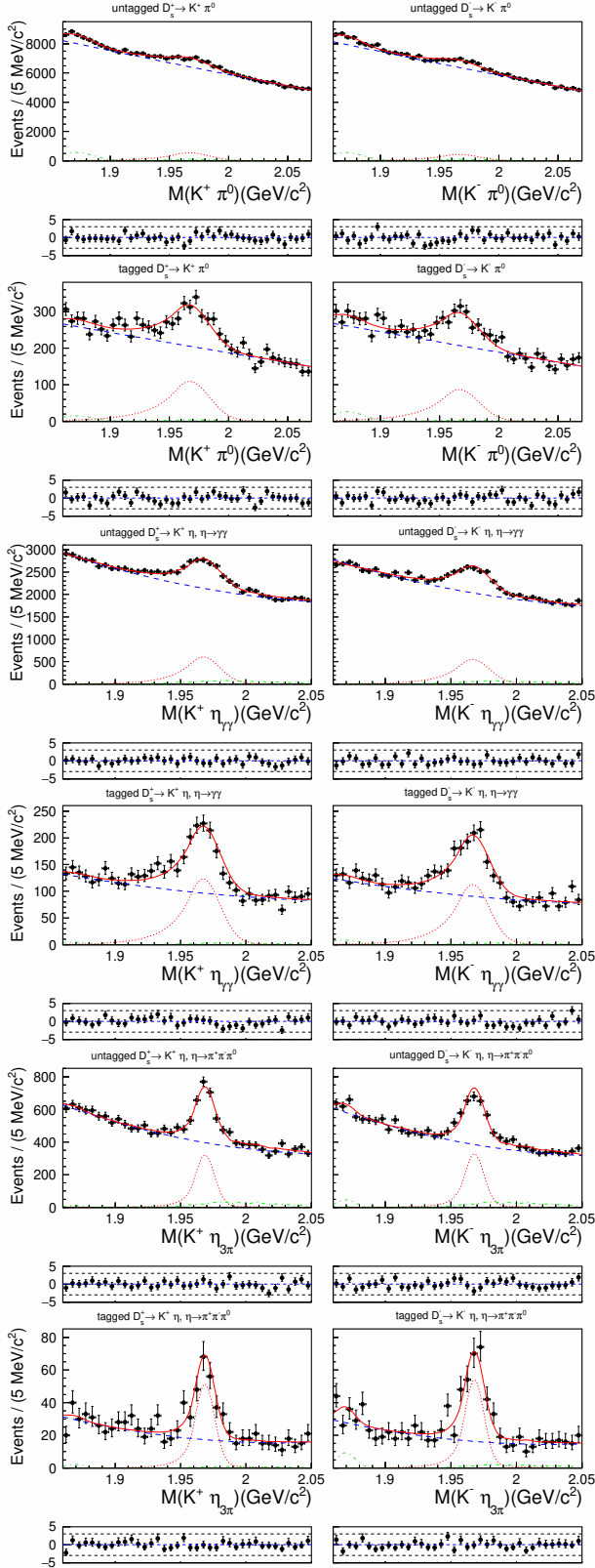
FIG. 1. (color online) Data and fit projection for D_s^+ \rightarrow K^+ \pi^0 (top two rows), D_s^+ \rightarrow K^+ \eta \gamma \gamma (middle two rows) and D_s^+ \rightarrow K^+ \eta_{3\pi} (bottom two rows). Left side shows D_s^+ candidates, right side shows D_s^- candidates. For each pair of rows, top is the untagged sample, bottom is the tagged sample. The red solid line is the total fit, the red dotted line is signal, the broken green line is background from D^+ , and the dashed blue line is combinatorial background. The plots beneath the distributions show the residuals.
