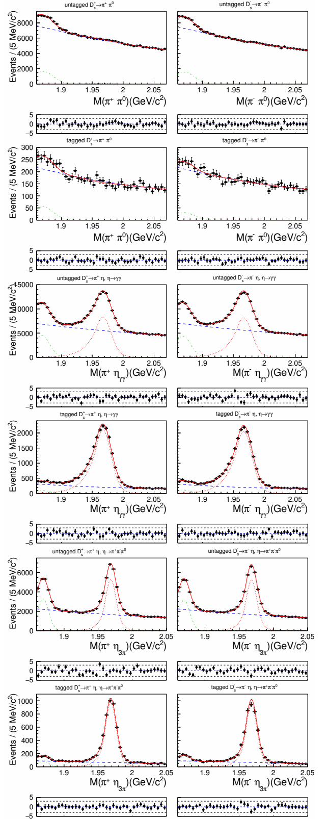
FIG. 2. (color online) Data and fit projection for D_s^+ \rightarrow \pi^+ \pi^0 (top two rows), D_s^+ \rightarrow \pi^+ \eta \gamma \gamma (middle two rows) and D_s^+ \rightarrow \pi^+ \eta_{3\pi} (bottom two rows). Left side shows D_s^+ candidates, right side shows D_s^- candidates. For each pair of rows, top is the untagged sample, bottom is the tagged sample. The red solid line is the total fit, the red dotted line is signal, the broken green line is background from D^+ , and the dashed blue line is combinatorial background. The plots beneath the distributions show the residuals.
