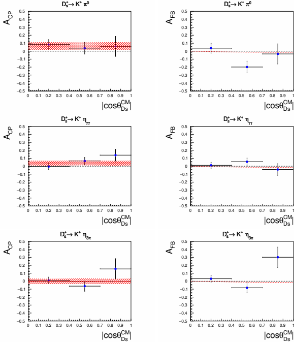
FIG. 4. (color online) CP asymmetries (left) and A_{FB} (right) in bins of |\cos \theta_{D_s}^{CM}| , for D_s^+ \rightarrow K^+ \pi^0 (top), D_s^+ \rightarrow K^+ \eta_{\gamma\gamma} (middle), and D_s^+ \rightarrow K^+ \eta_{3\pi} (bottom). In the left-side plots, the horizontal line shows the result of a fit to a constant, and the red shaded region shows the \pm 1\sigma errors. In the right-side plots, the dashed line shows the leading-order prediction [31].
