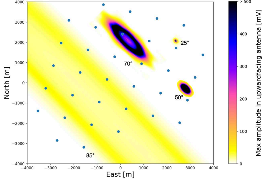
Figure 6. Simulated radio air shower footprints at 4 different incoming zenith angles. Simulations were performed using CORSIKA and the RNO-G site (magnetic field and height above sea level) in Greenland, and include the response of upward facing logarithmic periodic dipole antennas, as planned for RNO-G (see Fig. 7). The global maximum of the amplitudes in three antennas is shown. The air shower energy is 3.2 \times 10^{18} eV for all showers, and the zenith angles are indicated in the figure.
