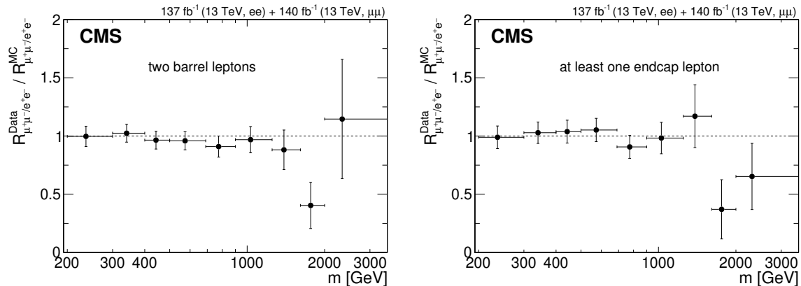
Figure 12: Ratio of the differential dilepton production cross section in the dimuon and dielectron channels R_{\mu^+\mu^-/e^+e^-} , as a function of m_{\ell\ell} for events with two barrel leptons on the left and at least one lepton in the endcaps on the right. The ratio is obtained after correcting the reconstructed mass spectra to particle level. The error bars include both statistical and systematic uncertainties.
