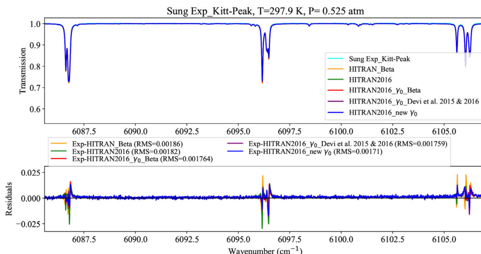
Fig. 16. The FTS transmission spectrum of CH 4 in the tetradecad region at P = 0.525 atm, T = 297.9 K, and X_{\text{CH}_4} = 0.01 (for a CH 4 -air mixture) measured at Kitt Peak National Solar Observatory (NSO). The top panel also shows calculated transmission spectra employing HAPI and the following data: i) the “HITRAN2016 Beta” line list, ii) the HITRAN2016 line list, iii) the HITRAN2016 line list with the broadening values collected from the “HITRAN2016 Beta” list, iv) the HITRAN2016 line list with the broadening parameters collected from Refs. [291,292], and v) the HITRAN2016 line list with the average broadening values obtained from Refs. [291,292]. The latter line list was eventually used for the HITRAN2020 update. The lower panel shows the differences between the experimental spectra and calculated transmission spectra using these line lists.
