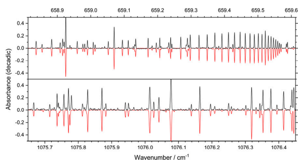
Fig. 31. Top panel: Experimental (upward) and simulated (downward) spectra of HCOOH within the \nu_9 fundamental using a Gaussian FWHM of 0.00171 \text{cm}^{-1} . Bottom panel: Experimental (upward) and simulated (downward) spectra spectra within the \nu_6 fundamental using a Gaussian FWHM of 0.00245 \text{cm}^{-1} .
