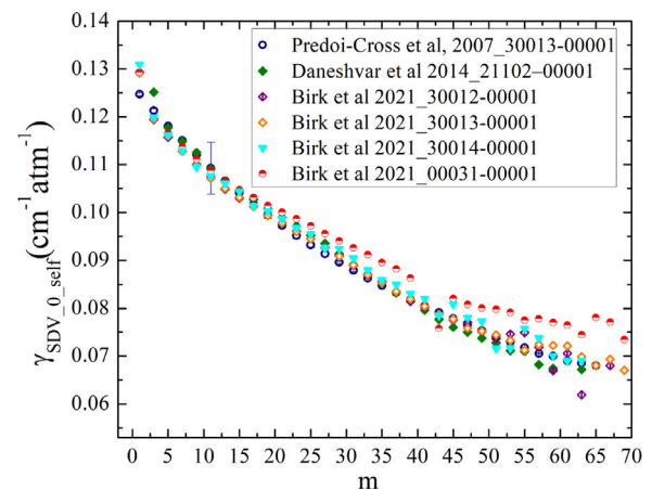
Fig. 6. The self-broadening parameters for CO 2 transitions at 296 K using the SDV profile. The values by Predoi-Cross et al. [176] are compared with the measurement of Ref. [177]. The Birk et al. [153] values are also presented for different bands.
