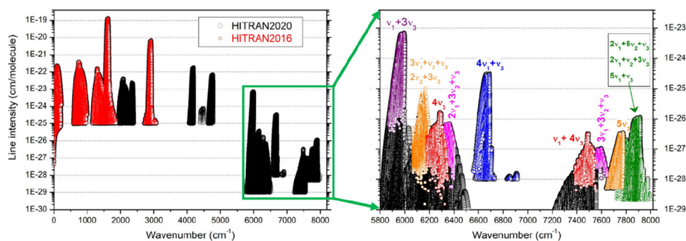
Fig. 23. Overview of the NO 2 line list for the main isotopologue, 14 N 16 O 2 . Left panel: Comparison of the HITRAN2016 and HITRAN2020 versions (red and black circles, respectively). Right panel: Enlargement of the 5800–8000 cm −1 region that has been updated using CRDS measurements. The HITRAN2020 update (black circles) has been overlaid by the original CRDS data for each band system [400–408], which are identified by color.
