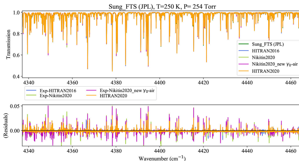
Fig. 15. The FTS transmission spectrum for CH 4 in the octad region at P = 254 Torr, T = 250 K, and X_{\text{CH}_4} = 0.0572 (for a CH 4 -air mixture) measured at JPL. The description for the lower panel is the same as in Fig. 14.
