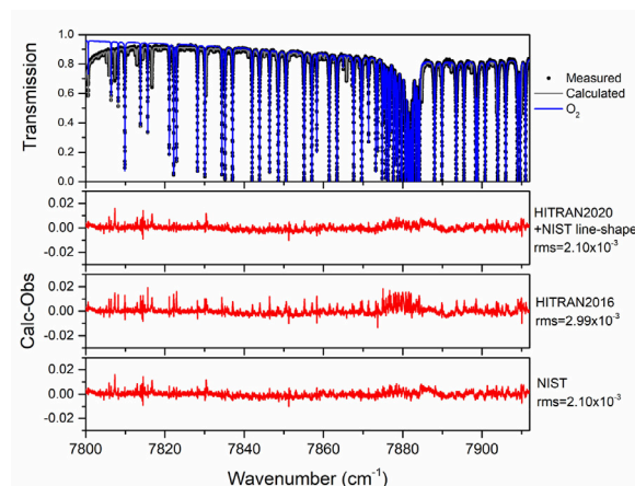
Fig. 17. Comparison between measured transmissions from Park Falls FTS and simulations using different versions of the database.
