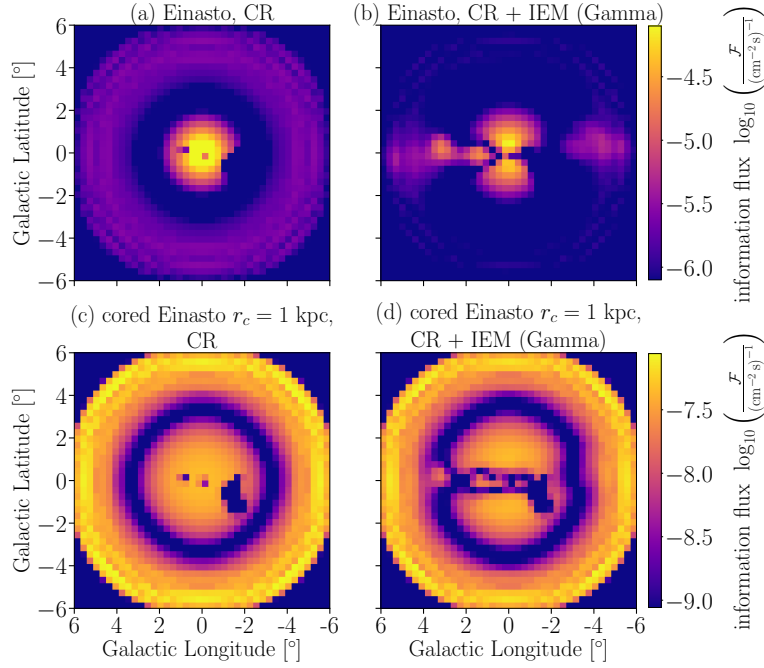
Figure 20. Left column: information flux \mathcal{F} (logarithmic colour scale), for Einasto (upper panel) and cored DM profiles (lower panel), assuming only the misidentified CR background (and no IE). Right column: same, but with the added emission based on the Gamma model. Regions with large \mathcal{F} yield most of the constraining power to a DM signal. These \mathcal{F} maps are based on the full GC survey, assuming our benchmark scheme of treating instrumental systematic uncertainties.
