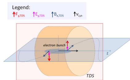
(a) Simplified sketch illustrating the direction of the dominant component of the electro-magnetic field in a RF-structure operating in the TM_{110} mode. In the represented case the deflection force acts in the vertical direction ( F_{y,TDS} ). B_x is the magnetic field component in the horizontal direction, E_y represents the electric field component in the transverse direction, v_{z,e} is the electron velocity.
