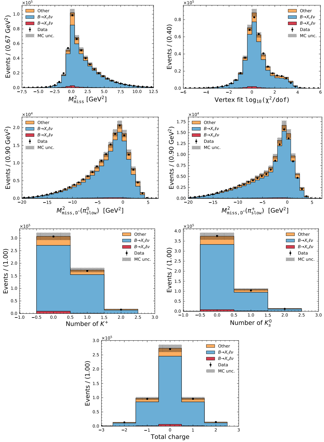
FIG. 15. The input variables for the B \rightarrow X_c \ell^+ \nu_\ell background suppression BDT for recorded and simulated events are shown. The uncertainty on the simulated events incorporate the full systematic uncertainties detailed in Section V.
