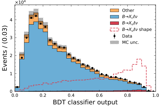
FIG. 4. The shape of the background suppression classifier \mathcal{O}_{\text{BDT}} is shown. MC is divided into B \rightarrow X_u \ell^+ \nu_\ell signal, the dominant B \rightarrow X_c \ell^+ \nu_\ell background, and all other contributions. To increase visibility, the B \rightarrow X_u \ell^+ \nu_\ell component is shown with a scaling factor (red dashed line). The uncertainties on the MC contain the full systematic errors and are further discussed in Section V.
