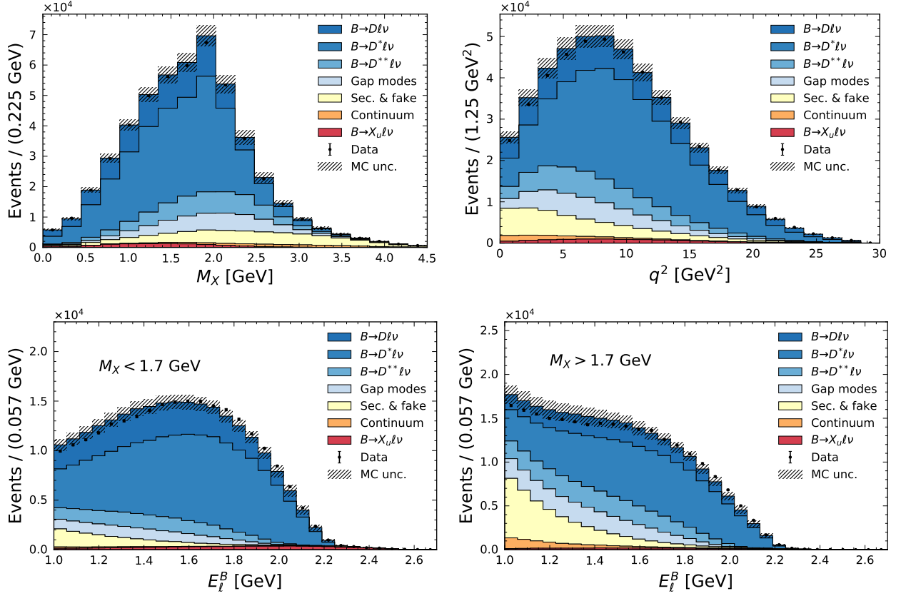
FIG. 5. (Top) The M_X and q^2 spectra of the selected candidates prior to applying the background BDT are shown. (Bottom) The E_\ell^B spectrum of the selected candidates prior to applying the background BDT are shown for events with M_X < 1.7 GeV and M_X > 1.7 GeV.
