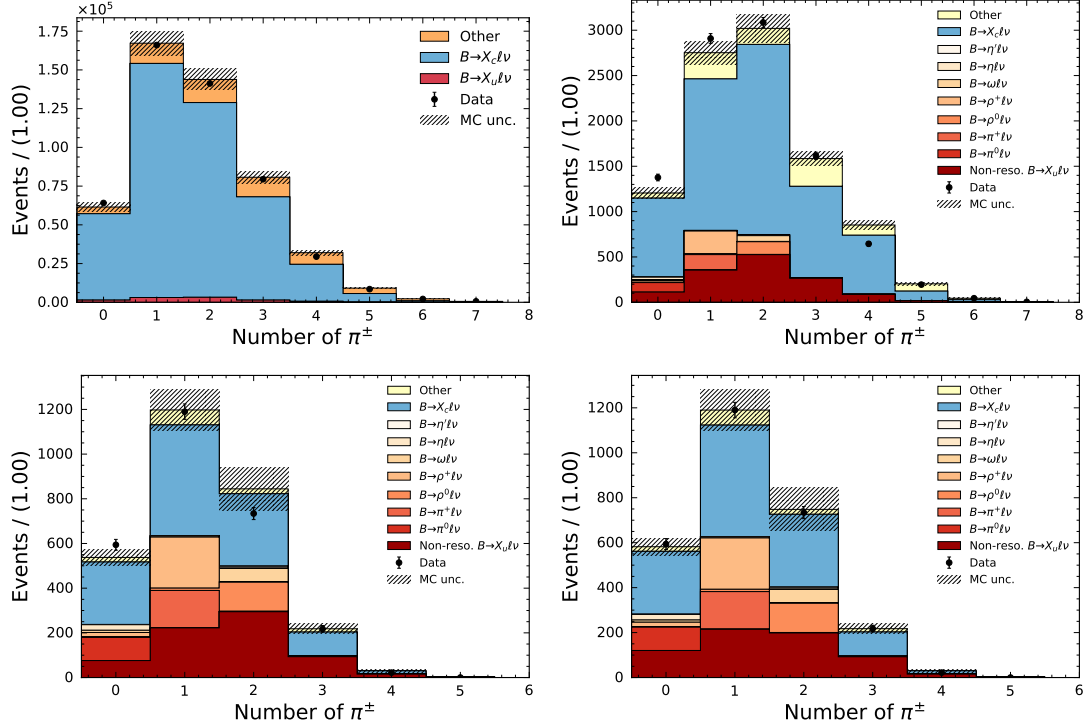
FIG. 18. The charged pion multiplicity ( n_{\pi^\pm} ) are compared between data and the simulation: (top left) for all events prior the BDT selection; (top right) for all events after the BDT selection; (bottom left): for the signal enriched region of M_X < 1.7 GeV; (bottom right) for the same region but after rescaling the non-resonant contributions such that the n_{\pi^\pm} fragmentation probability to match the one observed in data.
