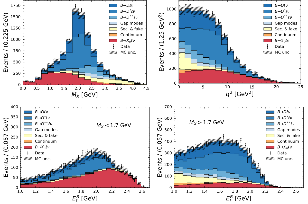
FIG. 6. The M_X , q^2 and E_\ell^B spectra after applying the background BDT but before the fit are shown. The B \rightarrow X_u \ell^+ \nu_\ell contribution is shown in red and scaled to the world average of \mathcal{B}(B \rightarrow X_u \ell^+ \nu_\ell) = (2.13 \pm 0.30) \times 10^{-3} . The data and MC agreement is reasonable in all variables. The E_\ell^B spectra is shown with selections of M_X < 1.7 GeV and M_X > 1.7 GeV. The cut of M_X < 1.7 GeV is later used in the fit to reduce the dependence on the B \rightarrow X_c \ell^+ \nu_\ell modeling of higher charmed states.
