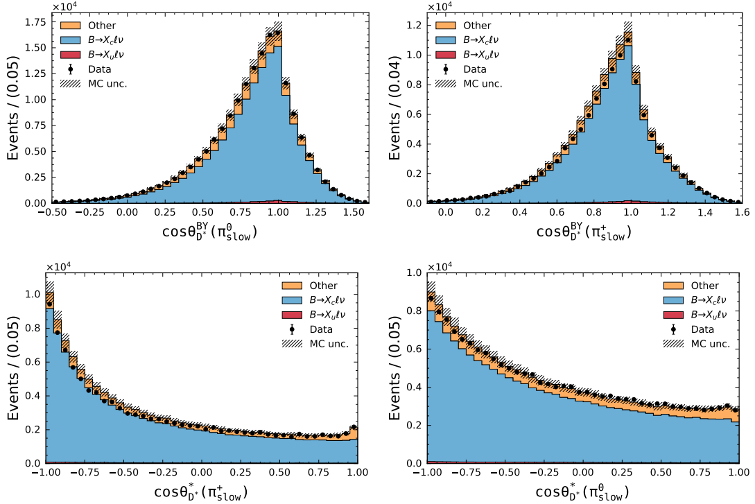
FIG. 17. The input variables for the B \rightarrow X_c \ell^+ \nu_\ell background suppression BDT for recorded and simulated events are shown. The uncertainty on the simulated events incorporate the full systematic uncertainties detailed in Section V.
