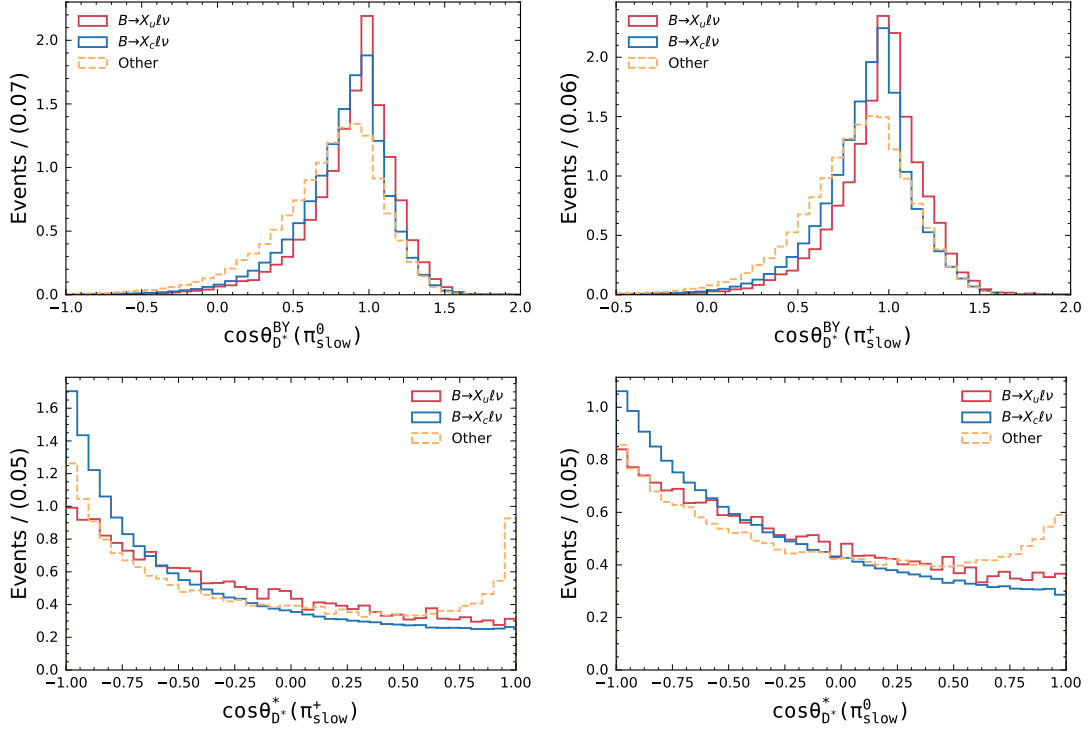
FIG. 16. The shape of the input variables for the B \rightarrow X_c \ell^+ \nu_\ell background suppression BDT are shown. For details and definitions see Section III C.
