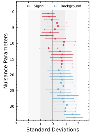
FIG. 20. The nuisance parameter pulls on the 2D fit of M_X : q^2 is shown.
