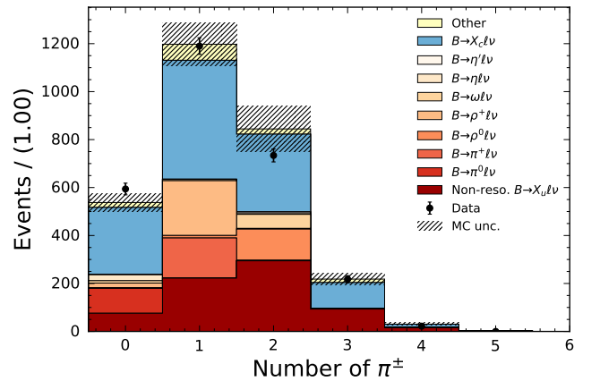
FIG. 11. The post-fit charged pion multiplicity is shown for events with M_X < 1.7 \text{ GeV} . The uncertainties on the MC stack include all systematic uncertainties.
