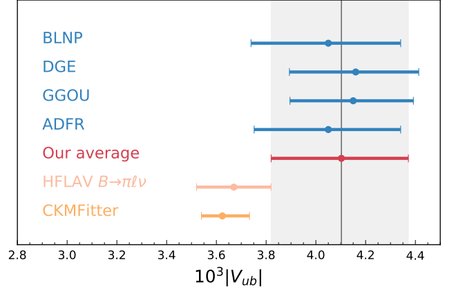
FIG. 12. The obtained values of |V_{ub}| from the four calculations and the arithmetic average is compared to the determination from exclusive B \rightarrow \pi \ell^+ \nu_\ell and the expectation from CKM unitarity [73] without the direct constraints from semileptonic and leptonic decays.
