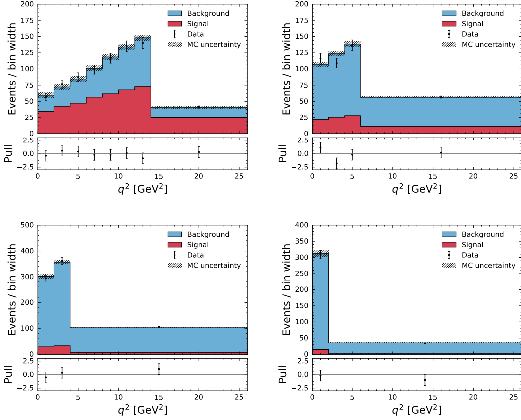
FIG. 21. The post-fit q^2 distributions of the two-dimensional fit to M_X : q^2 on M_X are shown. The panels correspond to: M_X \in [0, 1.5] GeV (top left), M_X \in [1.5, 1.9] GeV (top right), M_X \in [1.9, 2.4] GeV (bottom left) and M_X \in [2.4, 4] GeV (bottom right). The resulting yields are corrected to correspond to a partial branching fraction with E_\ell^B > 1 GeV.
