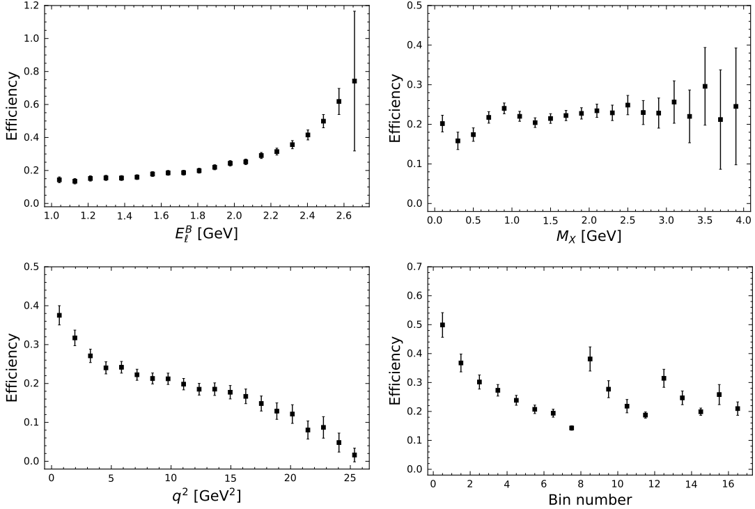
FIG. 22. The B \rightarrow X_u \ell^+ \nu_\ell efficiency after the BDT selection is shown as a function of the reconstructed kinematic variables ( E_\ell^B , M_X , q^2 ) used in the signal extraction. The bottom right plot shows the efficiencies in the bins of M_X : q^2 and the binning can be found in the text. The uncertainties are statistical only.
