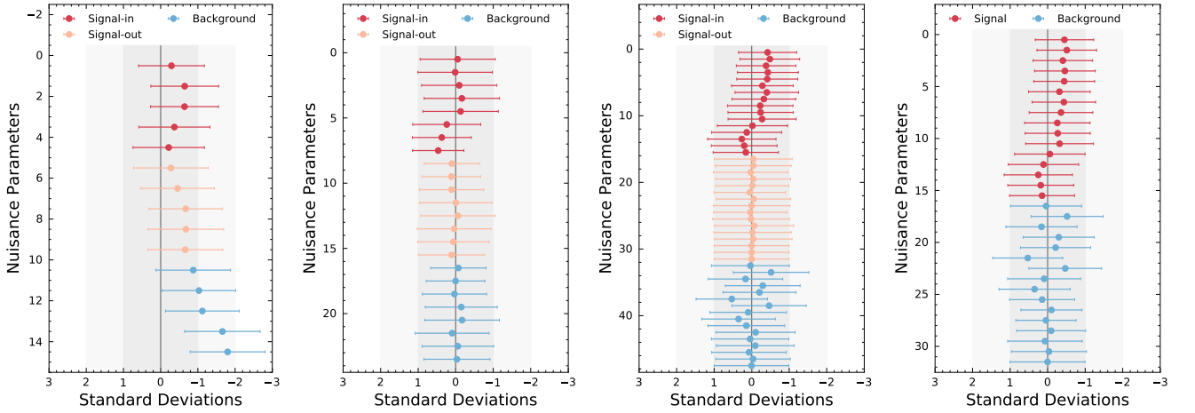
FIG. 19. The nuisance parameter pulls on the 1D fits of M_X , q^2 , and E_\ell^B with and without M_X < 1.7 GeV events separated out, are shown from left to right.
