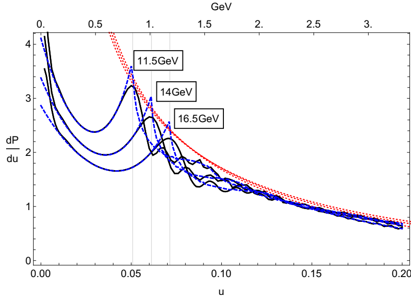
Figure A.2. Compton photon spectrum for three different electron energies and a \xi = 2 , laser pulse. The solid lines represent the full QED result [Eq. (27)], the blue dashed (red dotted) lines are the integration of the LMA [Eq. (31)] (LCFA [Eq. (28)]) rates. The vertical grid lines signify the position of the edge of the first harmonic (Compton edge) at intensity parameter \xi . (The photon energy scale in GeV on the upper horizontal axis is for 16.5 GeV electrons.)
