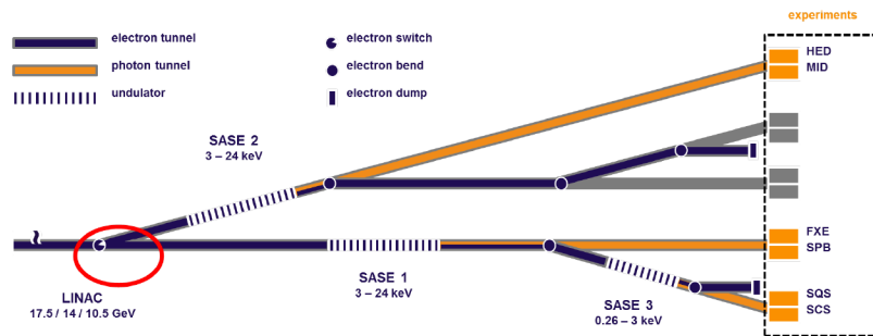
Figure 3.1. Schematic drawing of the XFEL.EU fan. The location foreseen of the LUXE experiment is circled in red. The SASE1, SASE2 and SASE3 undulators and the experimental halls are also shown.
