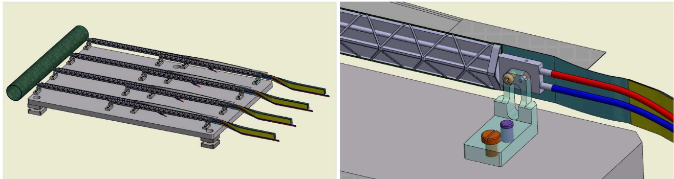
Figure 6.11. Left: one full tracker arm showing the flat tray and the L-shape bars used to fix the staves in their positions. Also shown in the picture is the beampipe. Right: A zoomed-in drawing of the L-shape bars.
