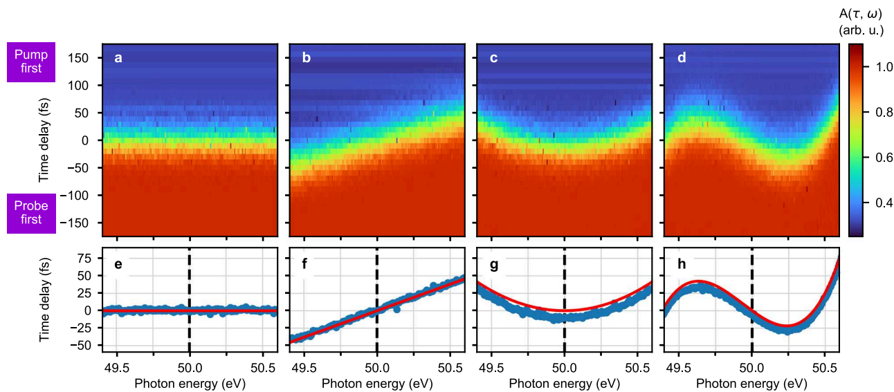
Fig. 2 Numerical simulation of the effect of plasma gating. a–d Calculated neon absorbance spectra for 50-fs SASE pulses, having averaged over 200 single SASE-FEL pulses per time-delay setting. Simulation for different values of D_n for n \geq 2 with increasing order from left to right. e–h The red solid curve represents the dispersion function \tau(\omega) , see Eq. (1), which was used as input for the calculation of the absorbance and corresponding output data (blue dots) are extracted by fitting a step function to the calculation results. The dashed vertical line indicates the 50-eV center photon energy (bandwidth around 1 eV). In the trivial case of no dispersion, i.e., D_n = 0 for n \geq 2 , displayed in a, e , the absorption spectrum is governed by a time-dependent “ramp” signal located at around \tau = 0 (pump-probe pulse overlap) and is constant over \omega . The case of a second-order (group-delay) dispersion of D_2 = 50 \text{ fs}^2 , displayed in b, f , yields a steep linear dependence of \tau(\omega) . c, g Parabola-shaped signal trace obtained through imposing a third-order dispersion of D_3 = 100 \text{ fs}^3 , and, displayed in d, h , the “wavy”-shaped signal trace obtained through a dominant fourth-order dispersion (combined dispersion coefficients D_2 = -100 \text{ fs}^2 , D_3 = 100 \text{ fs}^3 and D_4 = 1000 \text{ fs}^4 ). See Table 1 for quantitative analysis of numerical input and retrieved data.
