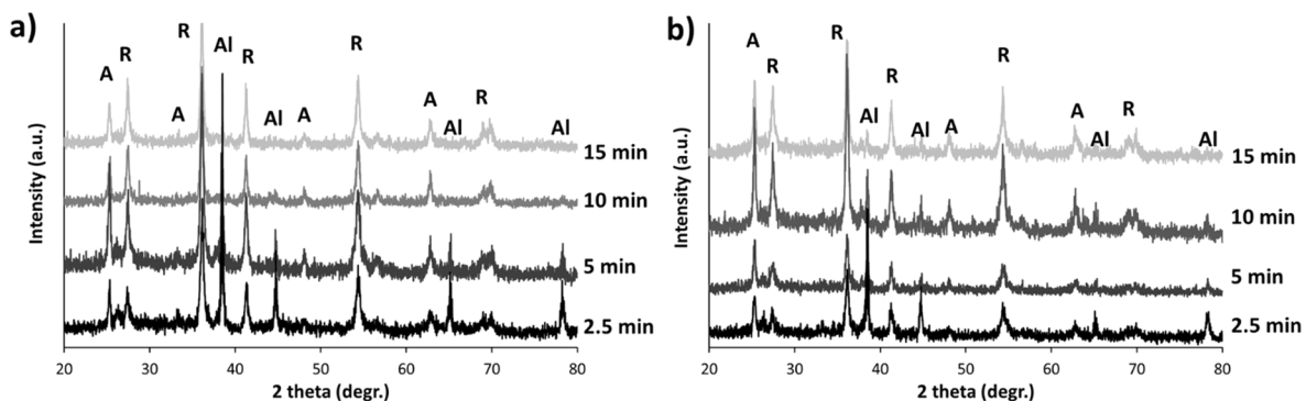
Fig. 10. XRD results of a) PEO coatings without Anatase – 2.5, 5, 10, 15 min treatment time and b) PEO coatings with 5 g/L Anatase particle addition – 2.5, 5, 10, 15 min treatment time. “R” indicates rutile, “A” – anatase, “Al” – AA2024 substrate.
