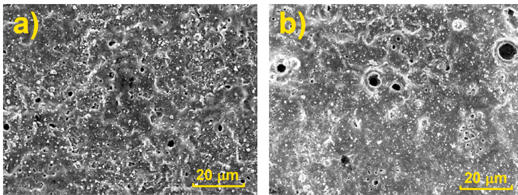
Fig. 9. Anatase particles deposited on the surface of the specimen – (a) 5 g/L anatase 5 min sample; (b) 5 g/L anatase 15 min sample.
