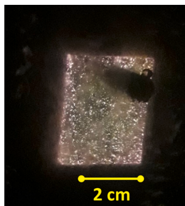
Fig. 4. Intense micro-discharges on surface of the metal alloy substrate during PEO processing in stage III.
