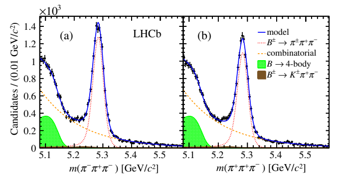
FIG. 1. Invariant-mass fit model for (a) B^- and (b) B^+ candidates reconstructed in the \pi^\pm \pi^+ \pi^- final state for the combined 2011 and 2012 data taking samples. Points with error bars represent the data while the components comprising the model are listed in the plot legend.
