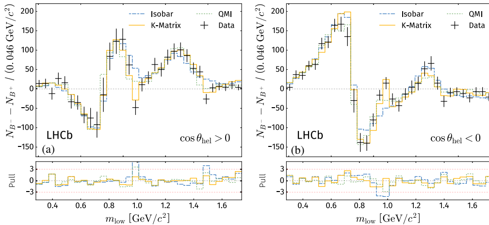
FIG. 12. Raw difference in the number of B^- and B^+ candidates in the low- m_{\text{low}} region, for (a) positive, and (b) negative cosine of the helicity angle. The pull distribution is shown below each fit projection.
