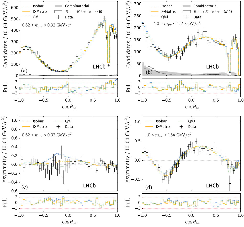
FIG. 9. Fit projections of each model on \cos \theta_{\text{hel}} (a) in the region around the \rho(770)^0 resonance and (b) in the f_2(1270) region, with the corresponding asymmetries shown beneath in panels (c) and (d). The pull distribution is shown below each fit projection.
