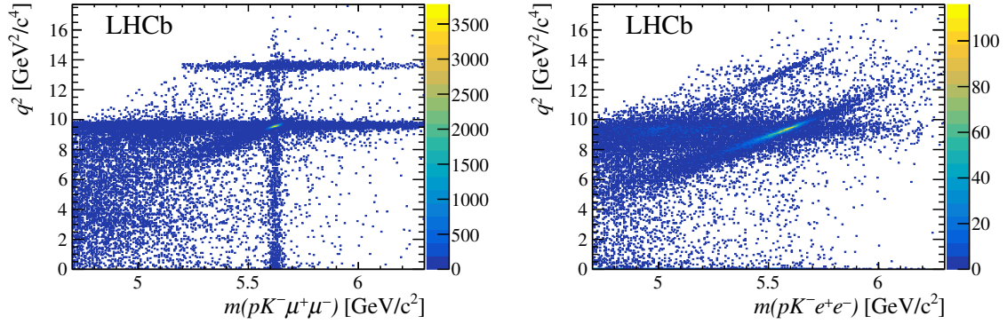
Figure 1. Distributions of dilepton invariant mass squared, q^2 , for \Lambda_b^0 candidates as a function of pK^-\ell^+\ell^- invariant mass, in data, for (left) \ell = \mu and (right) \ell = e . The complete selection is applied to both distributions, except for q^2 and m_{\text{corr}} requirements, defined in section 3.
