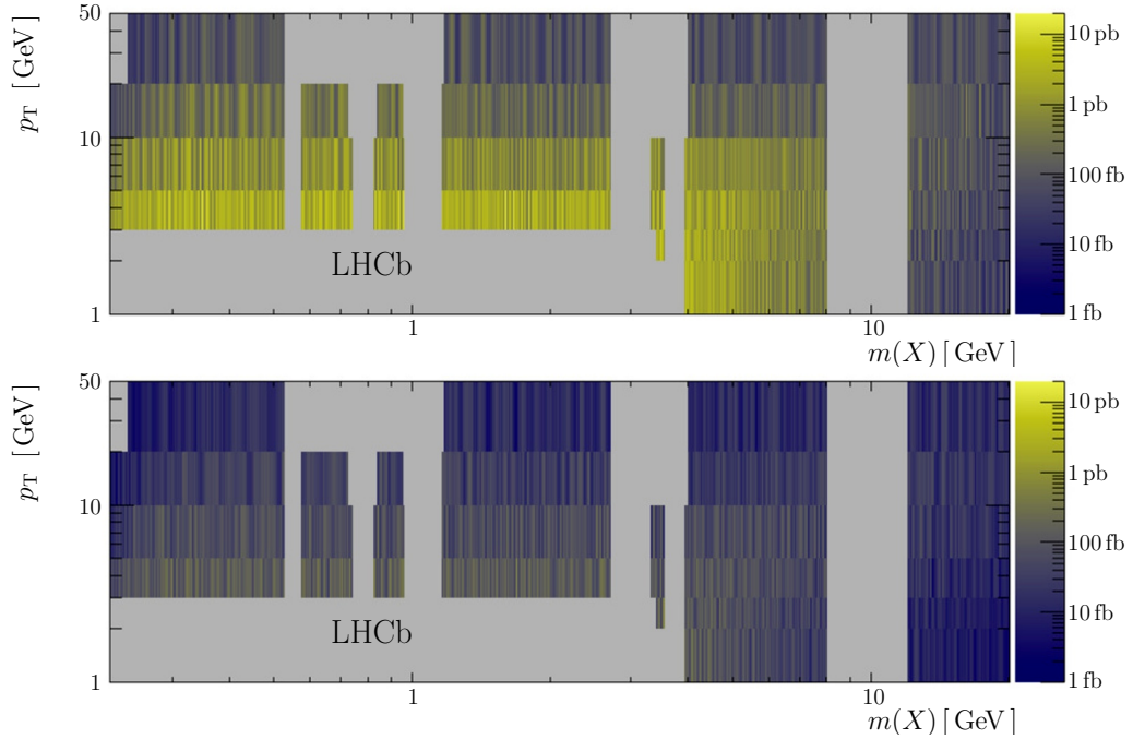
Figure 7. Upper limits at 90% confidence level on the cross section \sigma(X \rightarrow \mu^+\mu^-) in the m(X) < 20 GeV region for the (top) inclusive and (bottom) associated beauty searches for prompt X \rightarrow \mu^+\mu^- decays.
