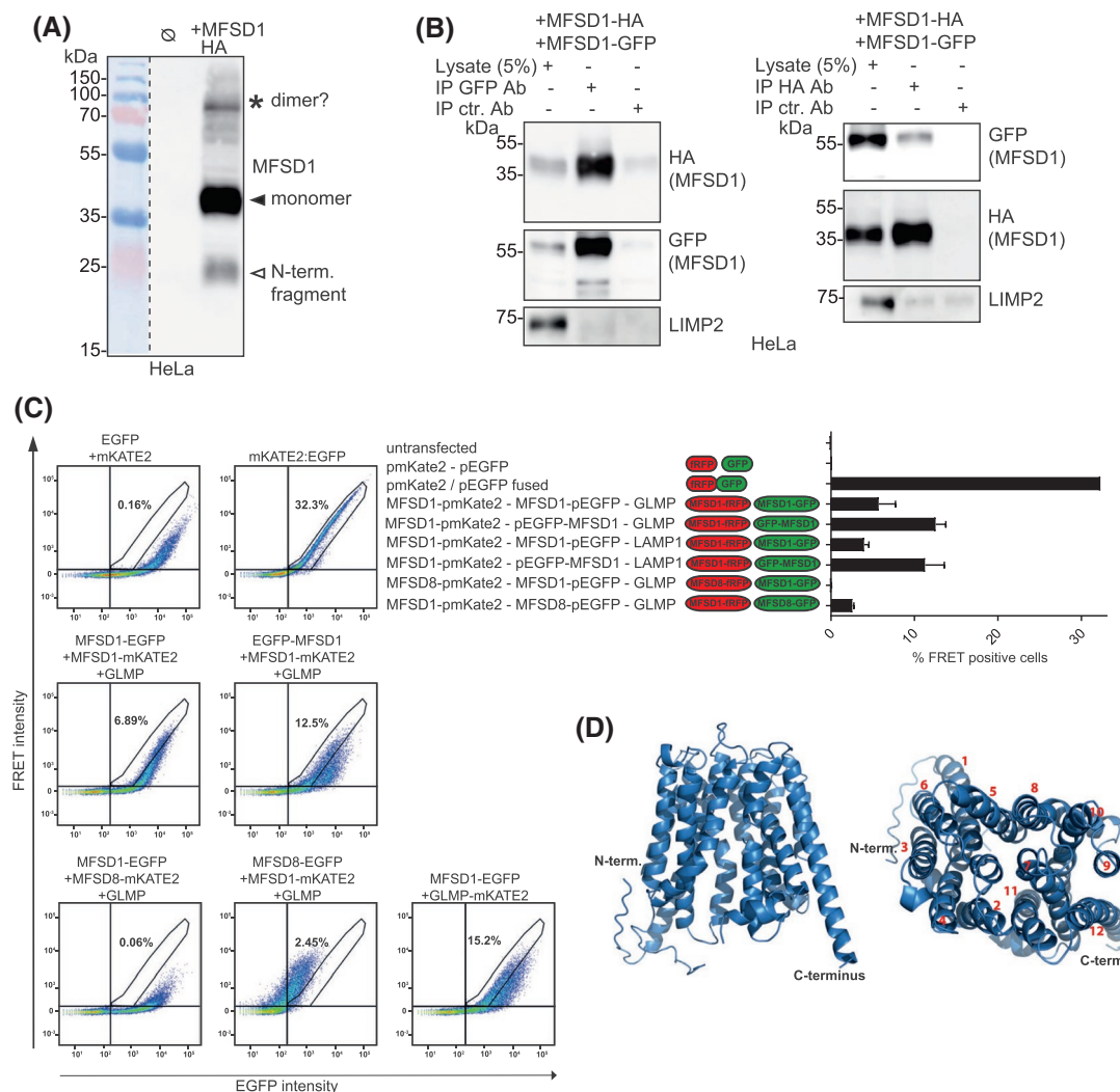
FIGURE 6 MFSD1 can form homodimers. A, Immunoblot analysis of HeLa cells overexpressing MFSD1-HA with an anti-HA antibody. A putative dimer is labeled with an asterisk. B, Immunoprecipitation of MFSD1-HA and MFSD1-GFP from transfected HeLa cells lysates transfected with both constructs using antibodies against HA and GFP. Co-immunoprecipitated proteins are detected with anti-HA and anti-GFP antibodies. Representative images from 2-3 independent experiments. C, Flow cytometry-based FRET analysis of HeLa cells transfected with combinations of plasmids coding for MFSD1, GLMP and MFSD8 untagged or tagged with eGFP or mKATE2. FRET intensity is plotted against eGFP intensity. Cells inside the gate defined by the intensity of cells expressing fused eGFP:mKATE2 were considered FRET+. The given numbers in the plot represents the average of alive FRET + cells for each condition, which is also represented in the bar graph. n = 3/ condition. D, Structure prediction of mMFSD1 using Phyre2 software with GLUT3 as a model. The prediction covers the mMFSD1 amino acid sequence from S20 to S451. Numbers in red represent the TMDs (1 = most N-terminal TMD, 12 most C-terminal TMD)
