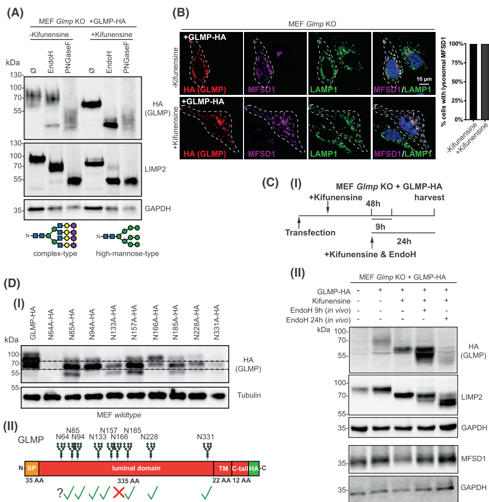
FIGURE 2 High-mannose type N-glycosylated GLMP can rescue MFSD1. A, Immunoblot analysis with the anti-HA antibody of Glmp KO MEF transfected with HA-tagged GLMP untreated or treated in vivo with the mannosidase I inhibitor kifunensine. Cell lysates were treated in vitro with EndoH or PNGaseF. LIMP2, which contains both high-mannose-type and complex-type glycans is shown as a positive control for the kifunensine-, EndoH-, and PNGaseF-treatment. GAPDH is depicted as a loading control. The N-glycan structures of complex-type glycans (left) and high-mannose-type glycans (right), the latter resulting from kifunensine-treatment, are schematically depicted below the immunoblot (blue square = N-Acetyl-D-glucosamine; green circle = mannose; yellow circle = galactose; magenta hexagon = neuraminic acid). B, Immunofluorescence for endogenous MFSD1 (purple) in Glmp KO MEFs transfected with GLMP-HA (red). Cells were untreated or incubated in vivo with kifunensine. The lysosomal marker LAMP1 is depicted in green. Nuclei are stained with DAPI (blue). Transfected cells are encircled with a dashed line. The percentage of cells with lysosomal MFSD1 staining pattern is diagramed (35–40 cells). C, (I) Schematic representation of the kifunensine/EndoH in vivo experimental setup. (II) Immunoblot analysis of GLMP-deficient MEFs transfected with HA-tagged GLMP untreated or treated with kifunensine and EndoH with the anti-HA antibody. LIMP2 is shown as a positive control for the kifunensine- and EndoH-treatment. Endogenous MFSD1 was detected with an MFSD1-specific antibody. GAPDH is depicted as a loading control. D, (I) Immunoblot analysis of wild-type MEFs overexpressing GLMP-HA or GLMP-HA with N/A mutations in the nine putative N-glycosylation sites detected with the anti-HA antibody. (II) Schematic representation of N-glycosylated asparagine residues in the luminal domain of GLMP. (A)–(C): Representative images from three independent experiments
