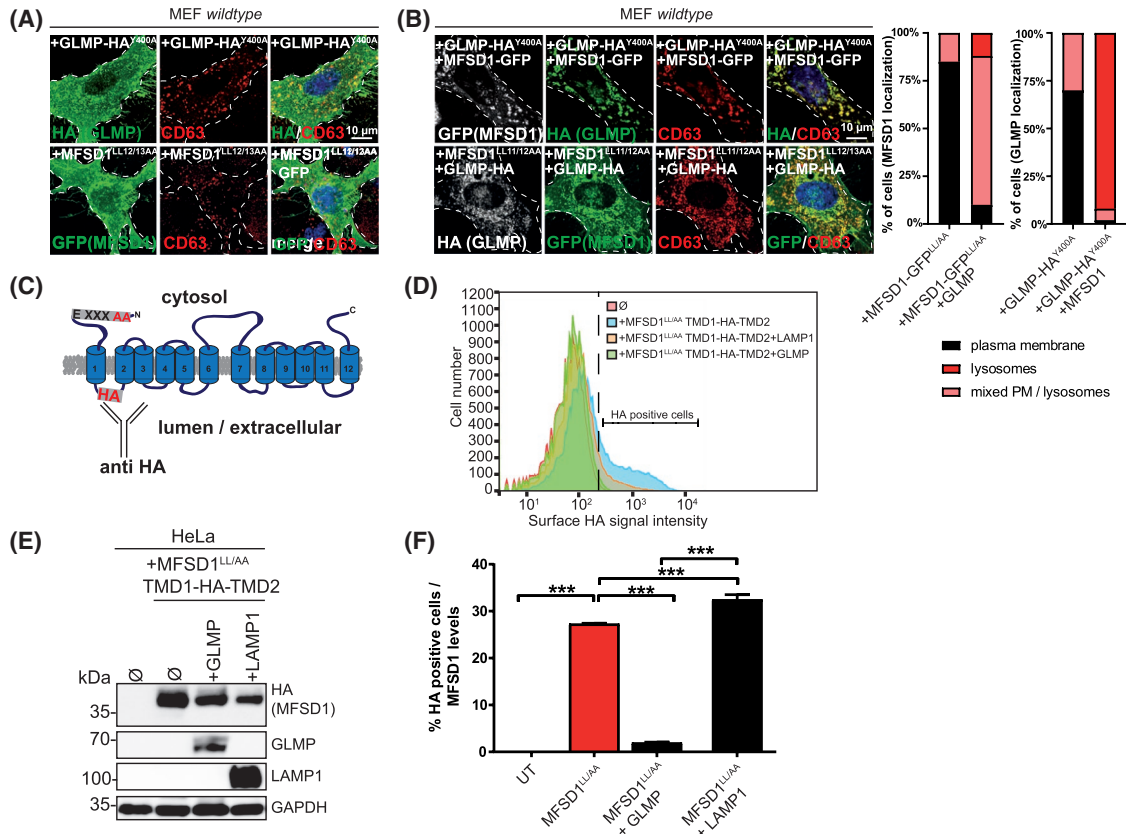
FIGURE 3 GLMP can deliver plasma-membrane targeted MFSD1 to lysosomes and vice versa . A, Immunofluorescence analysis of wild-type MEFs expressing GLMP Y/A -HA mutant (green) or MFSD1 LL/AA -GFP mutant (green) co-stained with the lysosomal marker CD63 (red). Nuclei are stained with DAPI (blue). Transfected cells are encircled with a dashed line. B, Immunofluorescence analysis of MEFs expressing GLMP Y/A -HA mutant (green) together with MFSD1-GFP (white) or MFSD1 LL/AA -GFP mutant (green) together with GLMP-HA (white) co-stained with the lysosomal marker CD63 (red). Nuclei are stained with DAPI (blue). Transfected cells are encircled with a dashed line. (A) - (B): Representative images from three independent experiments. The number of cells with MFSD1 LL/AA -GFP/ GLMP Y/A -HA at the plasma membrane, plasma membrane and lysosomes (mixed) or lysosomes is depicted (n = 30-40 cells). C, Schematic representation of the MFSD1 LL/AA -construct with an internal-HA-tag between TMD 1 and 2 (MFSD1 int LL/AA ) used for FACS analysis. D, FACS plots of untransfected HeLa cells, cells transfected with MFSD1 int LL/AA alone or together with LAMP1 or GLMP after staining of HA without permeabilization. E, Immunoblot analysis of untransfected HeLa cells, cells transfected with the MFSD1 int LL/AA alone or together with LAMP1 or GLMP, respectively. F, Quantification of the percentage of HA positive cells shown in (D) normalized to the HA expression levels shown in (E) (two-tailed unpaired t test; Mean ± SEM, n = 5. *** P < .0001).
