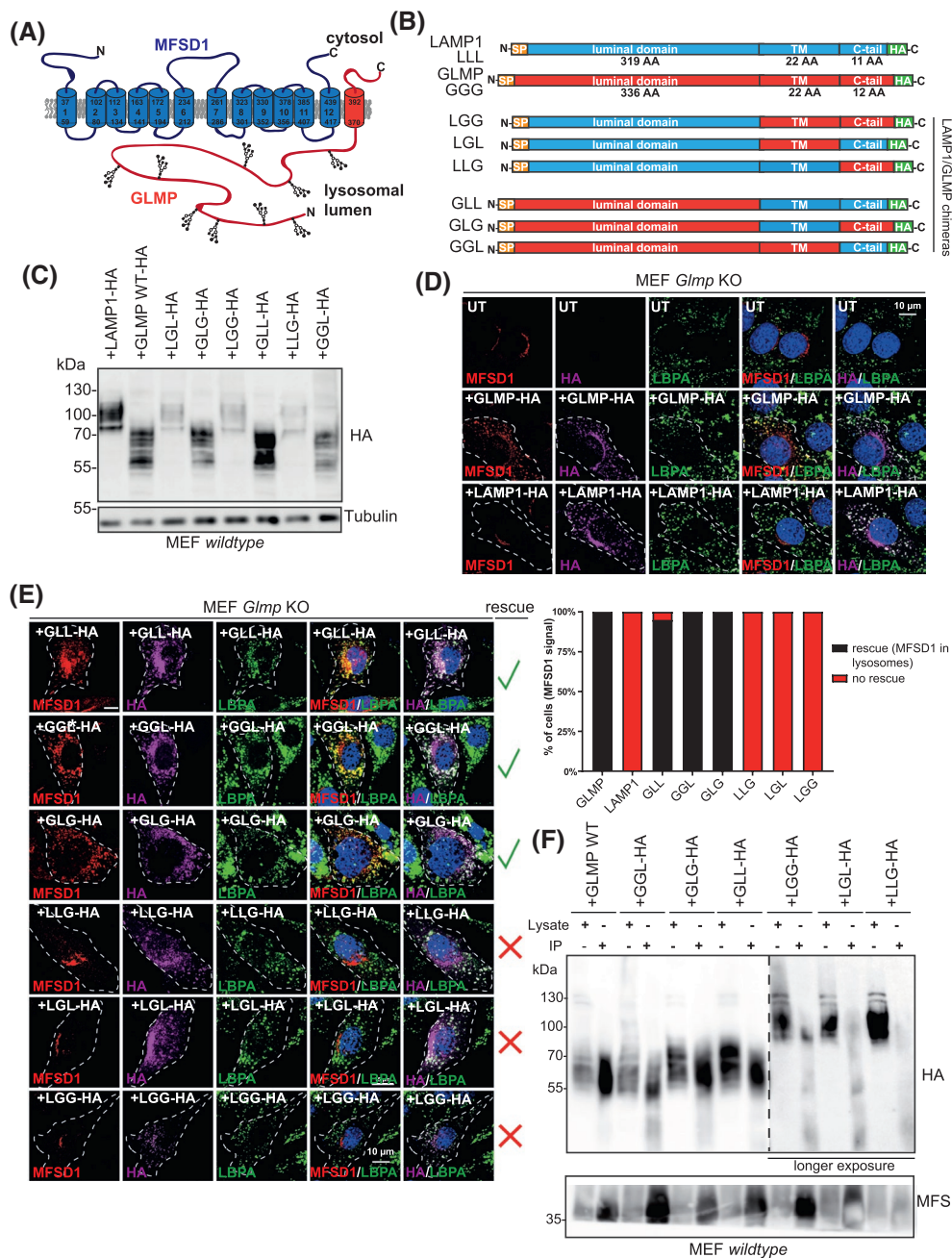
FIGURE 1 The luminal domain of GLMP interacts with MFSD1. A, Schematic representation of the molecular complex of MFSD1-GLMP. B, Schematic representation of HA-tagged chimeras of the cytosolic tail, the transmembrane domain and the luminal domain of GLMP and LAMP1. Abbreviations for the different chimeras are depicted on the left. (G = GLMP; L = LAMP1) C, Immunoblot analysis of the HA-tagged GLMP/LAMP1 chimeras expressed in wild-type MEFs detected with an antibody against HA. Tubulin is depicted as a loading control. D, Immunofluorescence staining for endogenous MFSD1 (red) in untransfected Glmp KO MEFs, cells transfected with GLMP-HA or LAMP1 HA (magenta). The late endosomal/lysosomal marker LBPA is shown in green. Nuclei are stained with DAPI (blue). Transfected cells are encircled with a dashed line. UT = untransfected. E, Expression of the HA-tagged GLMP/LAMP1 chimeras (magenta) in Glmp KO MEFs. Endogenous MFSD1 is depicted in red. LBPA, a late endosomal lipid, is shown in green. Rescue of endogenous MFSD1 is indicated (green tick). Transfected cells are encircled with a dashed line. A quantification of the percentage of cells, in which expression of GLMP, LAMP1 or the chimeras rescues lysosomal MFSD1 is given (25-30 cells). F, Co-Immunoprecipitation of the HA-tagged GLMP/LAMP1 chimeras with MFSD1. MFSD1 was immunoprecipitated with a polyclonal antibody against MFSD1. The HA-tagged GLMP-HA, LAMP1-HA and the chimeras were detected with an antibody against HA. The right part with LGG, LGL, and LLG is shown at higher exposure, as these chimeras were expressed at lower levels. Precipitation of MFSD1 detected on the membranes with the anti-MFSD1 antibody is shown in the lower panel. (C), (D) and (E): Representative images from three independent experiments
