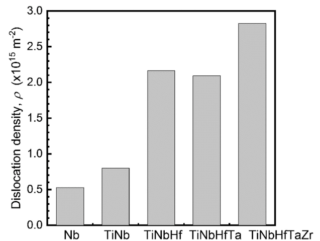
Fig. 4. Dislocation density accumulation in the as-swaged bcc Ti-Nb-Hf-Ta-Zr family samples.
