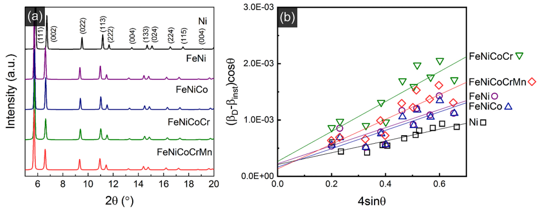
Fig. 1. (a) High energy synchrotron X-ray diffraction patterns and (b) Williamson-Hall plots of the as-swaged fcc Fe-Ni-Co-Cr-Mn family samples.
