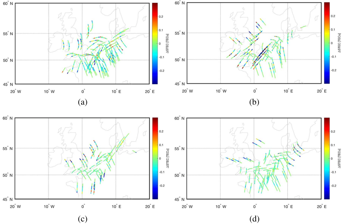
Fig. 15. Hourly geographical distribution of all STEC perturbations in the evening of 18 August 2013: (a) 18:00–19:00 UT, (b) 19:00–20:00 UT, (c) 20:00–21:00 UT, and (d) 21:00–22:00 UT.
