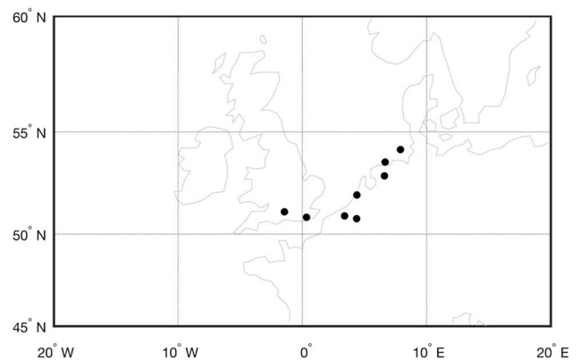
Fig. 13. Map showing the locations of the GNSS stations used.
