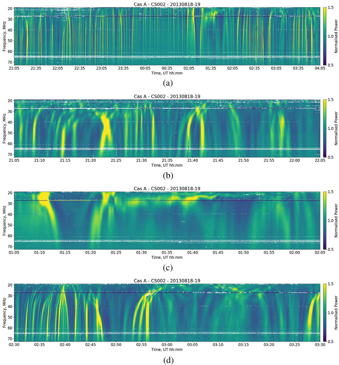
Fig. 2. Dynamic spectra of normalised intensity data taken by LOFAR station CS002 during the observation of Cas A on 18–19 August 2013. The dynamic spectrum of the entire observing period is given at the top, with zooms into three different hours of observation below to illustrate the range of conditions seen. White areas within the plots indicate where RFI was identified.
