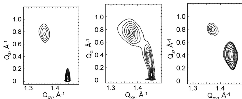
Fig. 6 GIXD data of 1- O -octadecyl- rac -glycerol monolayers on water at 5 °C, measured at 13 mN m -1 (left), 14 mN m -1 (middle) and 15 mN m -1 (right). The diffracted intensities, corrected for polarization, effective area, and Lorentz factor, are plotted as contour lines of equal intensity vs. the in-plane component Q_{xy} and the out-of-plane component Q_z of the scattering vector.
