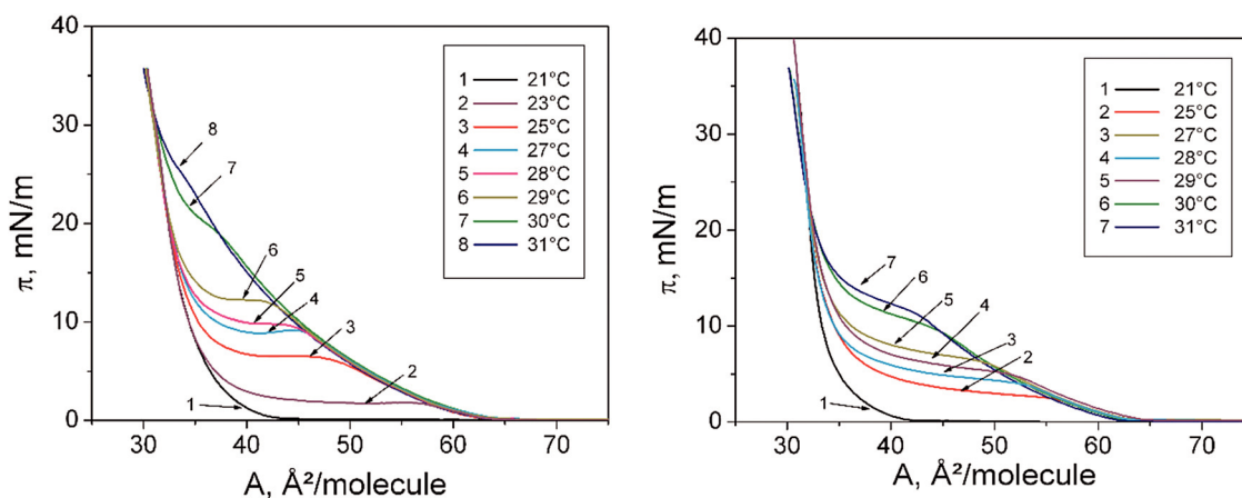
Fig. 2 \pi - A isotherms of the enantiomeric N -stearoyl-D- allo -threonine monolayers spread on pH 3 water and measured in the temperature range between 21 and 31 °C at compression (left) and at decompression (right).
