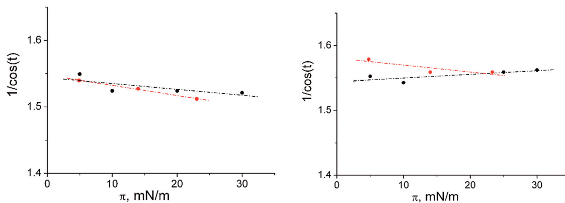
Fig. 7 Alkyl chain tilt angle (as 1/\cos(t) ) of N -stearoyl-allo-threonine vs. lateral pressure. Left: Enantiomeric C18 and right: racemic C18. The experimental points are red circles (●). For comparison, the corresponding values (black circles, ●) of N -stearoyl-D-threonine and racemic N -stearoyl-DL-threonine have been added.
