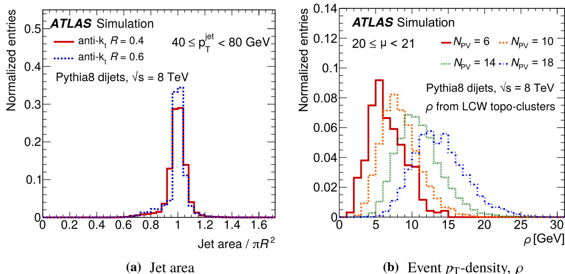
Fig. 3 a Ratio of the jet active area to \pi R^2 , where R is the jet radius parameter and b the event p_T -density \rho . The jet area ratio is shown separately for R = 0.4 and R = 0.6 jets reconstructed with the anti- k_t
