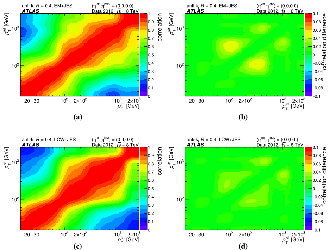
Fig. 45 The a, c JES correlation matrix and b, d difference between the full correlation matrix and that derived from a reduced number (6) of absolute in situ uncertainty components for anti- k_T , R = 0.4 jets calibrated with the a, b EM+JES and c, d LCW+JES schemes
