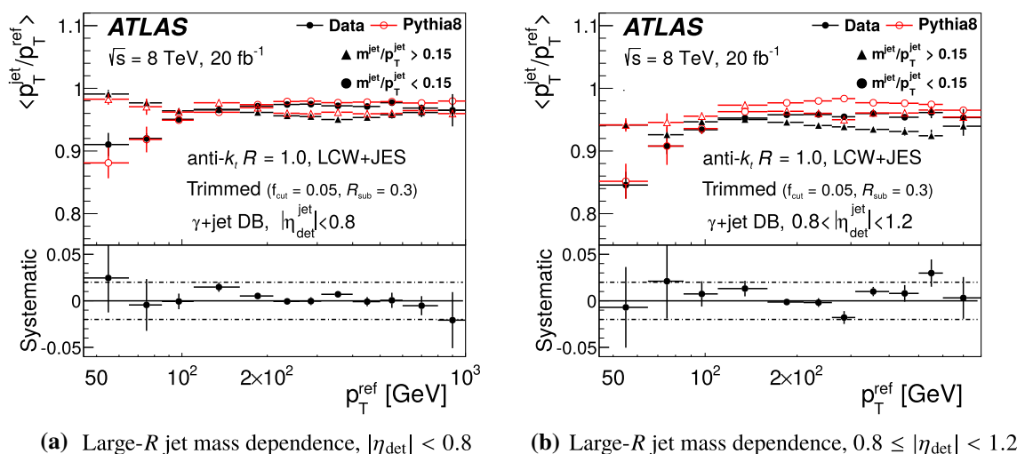
Fig. 30 R_{\text{DB}} as a function of p_T^{\text{ref}} measured for trimmed anti- k_t jets with R = 1.0 in \gamma +jet events shown separately for jets with a |\eta_{\text{det}}| < 0.8 and b 0.8 \leq |\eta_{\text{det}}| < 1.2 . Separate results are shown for jets with m/p_T < 0.15 and m/p_T > 0.15 , displayed with circles and triangles, respectively. Measurements in data are shown as filled
