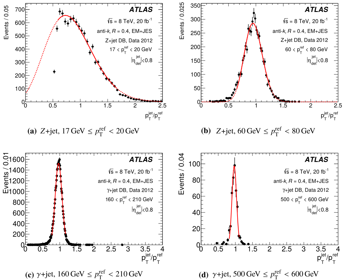
Fig. 21 Distributions of p_T^{\text{jet}}/p_T^{\text{ref}} for a 17 \text{ GeV} \leq p_T^{\text{ref}} < 20 \text{ GeV} , b 60 \text{ GeV} \leq p_T^{\text{ref}} < 80 \text{ GeV} , c 160 \text{ GeV} \leq p_T^{\text{ref}} < 210 \text{ GeV} , and d 500 \text{ GeV} \leq p_T^{\text{ref}} < 600 \text{ GeV} using anti- k_t jets with R = 0.4 calibrated with the EM+JES scheme in data from the a , b Z+jet and c , d \gamma +jet analyses. The dashed lines in a , b show the fitted Modified
