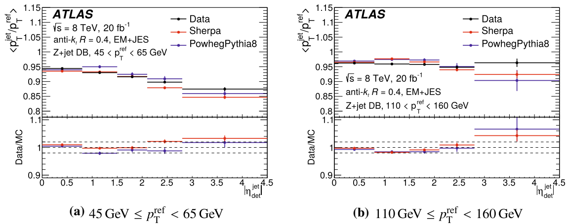
Fig. 23 R_{DB} as a function of \eta_{det} for anti- k_t jets with R = 0.4 calibrated with the EM + JES scheme in data (black), as well as in SHERPA (red) and POWHEG + PYTHIA8 (blue) simulation, for a 45 \text{ GeV} \leq p_T^{\text{ref}} < 65 \text{ GeV} and b 110 \text{ GeV} \leq p_T^{\text{ref}} < 160 \text{ GeV} . Only statistical uncertainties are shown
