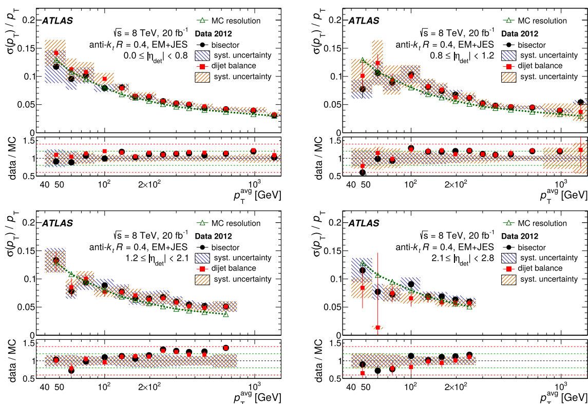
Fig. 20 Relative jet energy resolution obtained for EM+JES calibrated jets using the bisector (filled circles) and dijet balance (filled squares) methods, respectively. The MC simulated resolution derived from matching truth-particle jets with calorimeter jets is presented by the open triangles connected by dashed lines. The error bars reflect the
