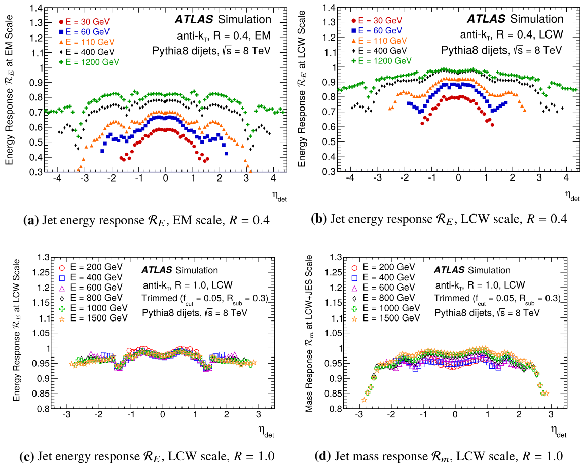
Fig. 4 Jet energy and mass responses as a function of \eta_{\text{det}} for different truth-particle jet energies. The energy responses \mathcal{R}_E for anti- k_t jets with R = 0.4 at the a EM scale and the b LCW scale and c for trimmed anti- k_t R = 1.0 jets are presented. Also, d the jet mass response \mathcal{R}_m for the latter kind of jets is given
