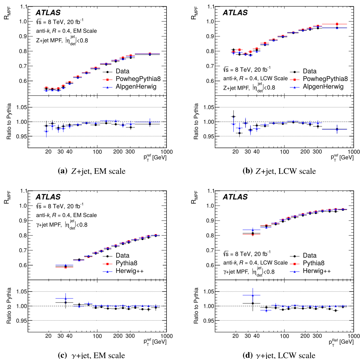
Fig. 24 The MPF response R_{\text{MPF}} in a, b Z+jet and c, d \gamma +jet events for jets calibrated a, c at the EM scale and b, d using the LCW scheme, for both data and MC simulation, as a function of p_T^{\text{ref}} . Only statistical uncertainties are shown
