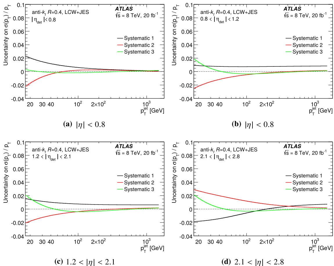
Fig. 56 The three eigenvectors after the eigenvector reduction of the nuisance parameters in the jet energy resolution measurement for LCW+JES R = 0.4 jets for four different |\eta| bins. These nuisance parameters fully describe the correlations
