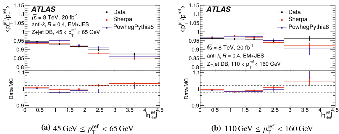
Fig. 23 R_{DB} as a function of \eta_{det} for anti- k_t jets with R = 0.4 calibrated with the EM+JES scheme in data (black), as well as in SHERPA (red) and POWHEG+PYTHIA8 (blue) simulation, for a 45 \text{ GeV} \leq p_T^{ref} < 65 \text{ GeV} and b 110 \text{ GeV} \leq p_T^{ref} < 160 \text{ GeV} . Only statistical uncertainties are shown
