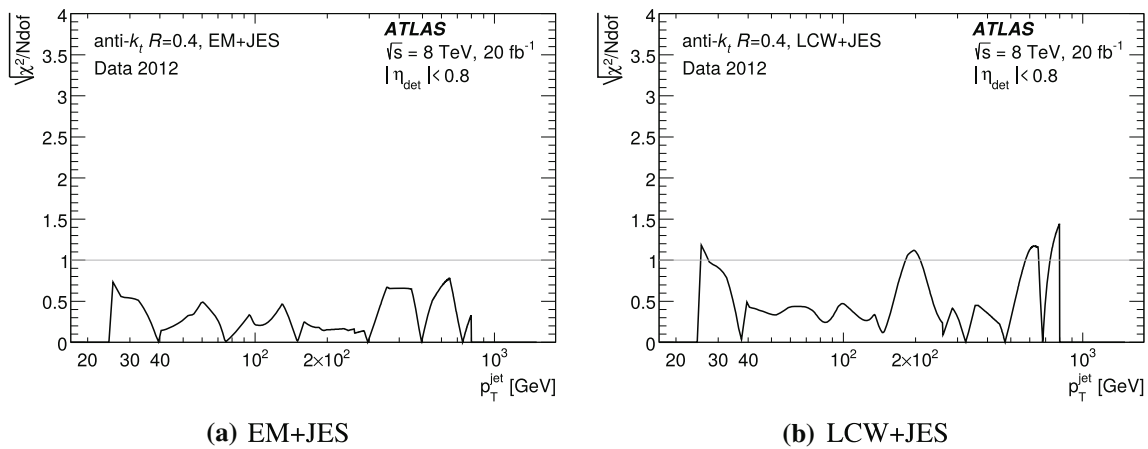
Fig. 55 The \chi^2 per degree of freedom for the jet energy resolution showing the compatibility of the three in situ measurements of the jet energy resolution (dijet asymmetry, Z+jet balance, and \gamma +jet balance) for jets calibrated with the a EM+JES and b LCW+JES schemes
