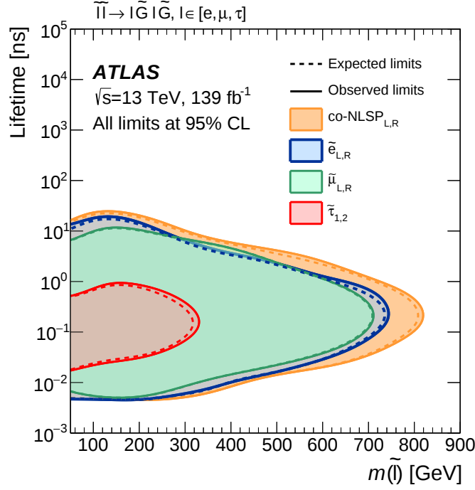
Figure 2: Expected (dashed) and observed (solid) exclusion contours for \tilde{e} NLSP, \tilde{\mu} NLSP, \tilde{\tau} NLSP, and co-NLSP production as a function of the slepton \tilde{\ell} mass at 95% CL. Selectrons, \tilde{e}_{L,R} , and smuons, \tilde{\mu}_{L,R} , are the superpartners of the left- and right-handed electrons and muons. Staus, \tilde{\tau}_{1,2} are the mixed states of the superpartners of the left- and right-handed \tau -leptons, with mixing angle \sin \theta_{\tilde{\tau}} = 0.95 . The different \tilde{\ell} chiral states are assumed to be mass degenerate.
