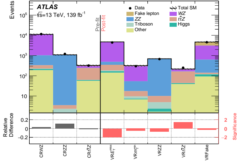
Figure 5: The observed data and the SM background expectation in the CRs (pre-fit) and VRs (post-fit). The “Other” category consists mostly of the tWZ , t\bar{t}W , and tZ processes. The hatched bands indicate the combined theoretical, experimental, and MC statistical uncertainties in the background prediction. The bottom panel shows the fractional difference between the observed data and expected yields for the CRs and the significance of the difference for the VRs, computed following the profile likelihood method described in Ref. [102].
