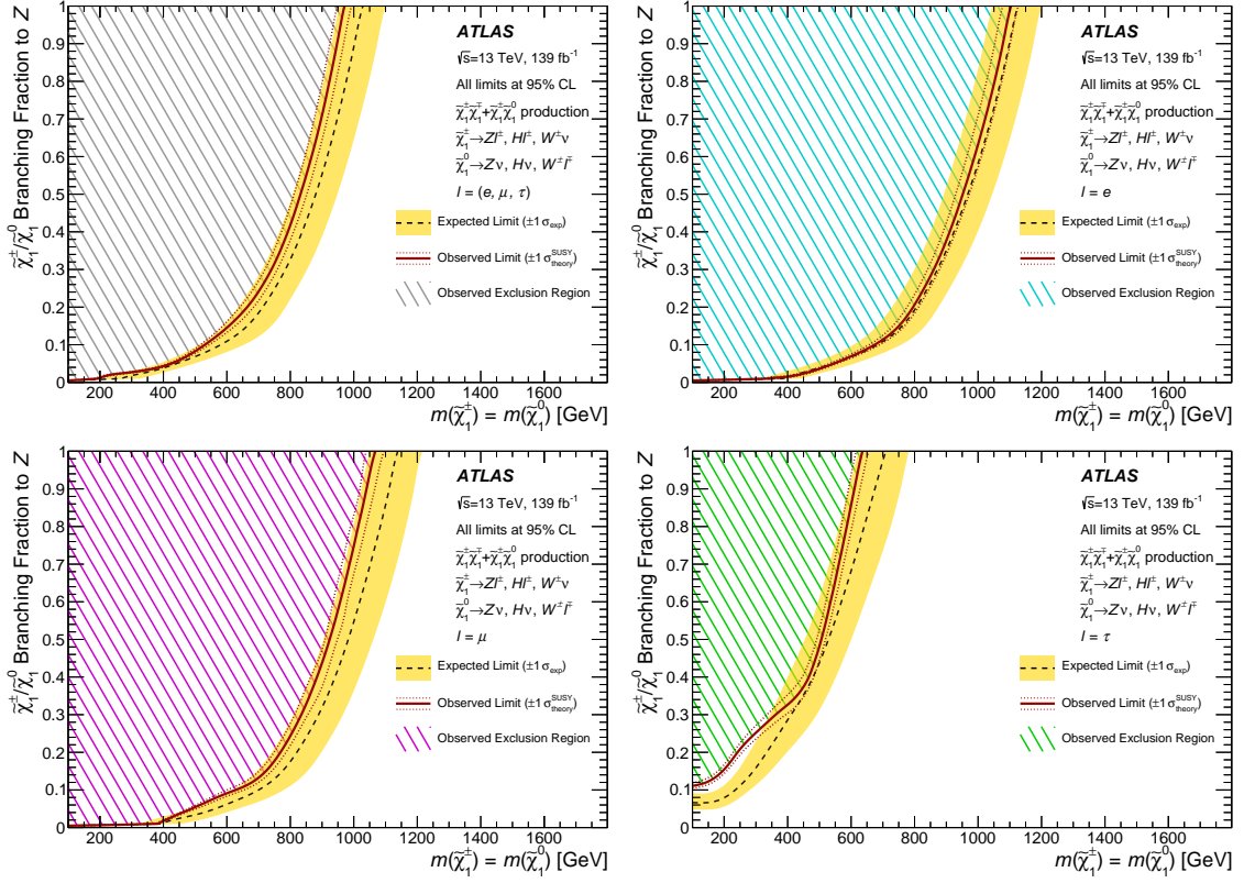
Figure 9: Exclusion curves for the simplified model of \tilde{\chi}_1^\pm \tilde{\chi}_1^\mp + \tilde{\chi}_1^\pm \tilde{\chi}_1^0 production as a function of \tilde{\chi}_1^\pm/\tilde{\chi}_1^0 mass and branching fraction to Z bosons. Curves are derived separately when requiring that the charged-lepton decays of \tilde{\chi}_1^\pm/\tilde{\chi}_1^0 are into (top left) any leptons with equal probability, (top right) electrons only, (bottom left) muons only, or (bottom right) \tau -leptons only. The expected 95% CL exclusion (dashed black line) is shown with \pm 1 \sigma_{\text{exp}} variations (shaded yellow band) from systematic and statistical uncertainties in the expected yields. The observed 95% CL exclusion (solid red line) is shown with \pm 1 \sigma_{\text{theory}}^{\text{SUSY}} variations (dotted red lines) from cross-section uncertainties for the signal models. The phase-space excluded by the search is shown in the hatched regions. The sum of the \tilde{\chi}_1^\pm/\tilde{\chi}_1^0 branching fractions to W, Z, and Higgs bosons is unity for each point, and the branching fractions to W and Higgs bosons are chosen so as to be equal everywhere.
