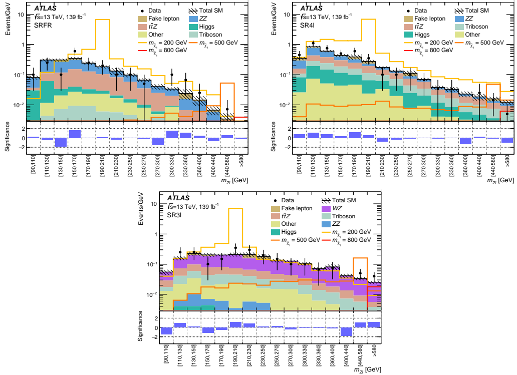
Figure 7: The observed data and post-fit SM background expectation as a function of m_{Z\ell} in (top left) SRFR, (top right) SR4 \ell , and (bottom) SR3 \ell . The m_{Z\ell} binning (Eq. (1)) is the same as that used in the fit and the yield is normalized to the bin width, with the last bin normalized using a width of 200 GeV. The “Other” category consists mostly of the tWZ , t\bar{t}W , and tZ processes. The hatched bands indicate the combined theoretical, experimental, and MC statistical uncertainties in the background prediction. The bottom panel shows the significance of the differences between the observed data and expected yields, computed following the profile likelihood method described in Ref. [102].
