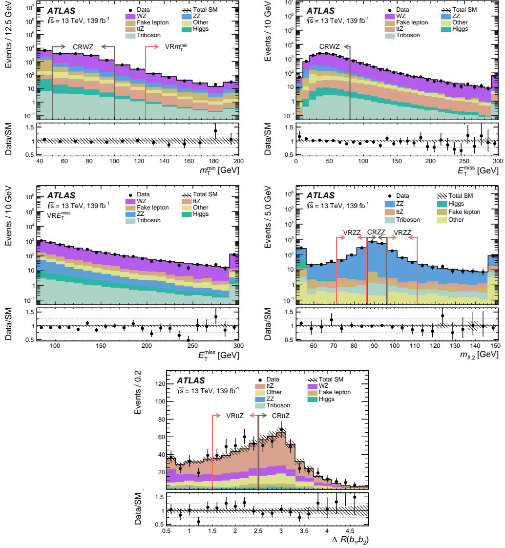
Figure 3: Distributions of the data and post-fit background in the CRs and VRs that are relevant in the extrapolation to the SRs, including (top left) m_T^{\text{min}} in CRWZ and VRm_T^{\text{min}} , (top right) E_T^{\text{miss}} in CRWZ, (middle left) E_T^{\text{miss}} in VRE_T^{\text{miss}} , (middle right) m_{\ell\ell,2} in CRZZ and VRZZ, and (bottom) \Delta R(b_1, b_2) in CRt\bar{t}Z and VRt\bar{t}Z . Black (red) arrows indicate the CR (VR) selection on the variable shown, with all other region selections applied. The first (last) bin includes underflow (overflow) events. The “Other” category consists mostly of the tWZ , t\bar{t}W , and tZ processes. The hatched bands indicate the combined theoretical, experimental, and MC statistical uncertainties in the background prediction. The bottom panel shows the ratio of the data to the background prediction.
