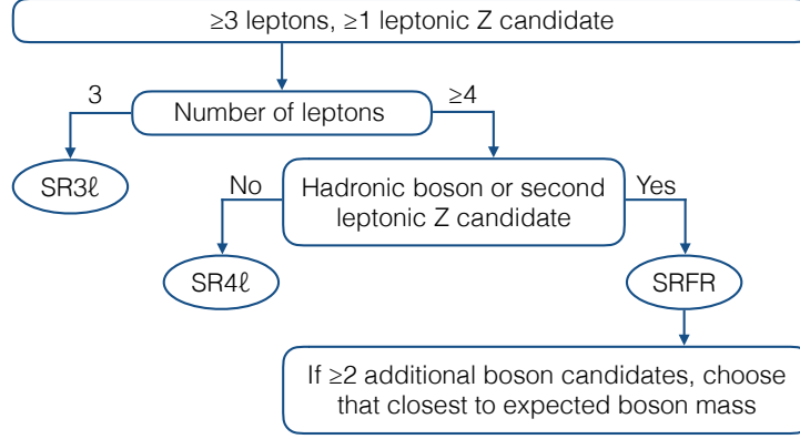
Figure 2: Schematic flow chart describing the assignment of an event to a given signal region.
