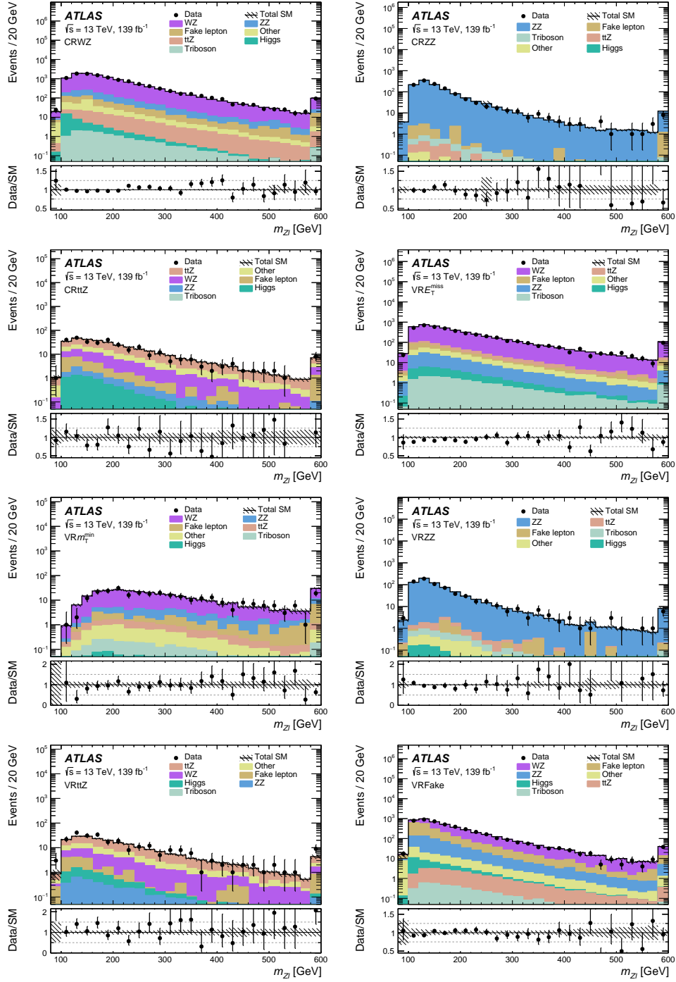
Figure 4: The m_{Zl} distributions of the data and post-fit background in the (from top left to bottom right) CRWZ, CRZZ, CR t Z, VRE_T^{\text{miss}} , VRm_T^{\text{min}} , VRZZ, VR t Z, and VRFake regions. The last bin includes overflow events. The “Other” category consists mostly of the tWZ , t\bar{t}W , and tZ processes. The hatched bands indicate the combined theoretical, experimental, and MC statistical uncertainties in the background prediction. The bottom panel shows the ratio of the data to the background prediction.
