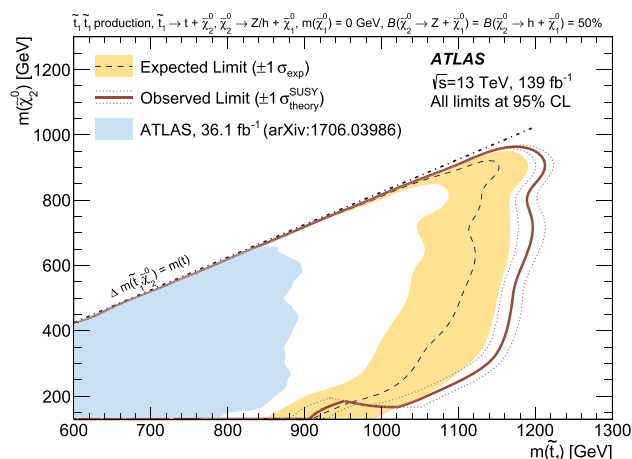
Fig. 10 Exclusion limits at 95% CL on the masses of the \tilde{t}_1 and \tilde{\chi}_2^0 , for a fixed m(\tilde{\chi}_1^0) = 0 GeV, assuming B(\tilde{\chi}_2^0 \rightarrow Z\tilde{\chi}_1^0) = 0.5 and B(\tilde{\chi}_2^0 \rightarrow h\tilde{\chi}_1^0) = 0.5 . The dashed line and the shaded band are the expected limit and its \pm 1\sigma uncertainty, respectively. The thick solid line is the observed limit for the central value of the signal cross-section. The expected and observed limits do not include the effect of the theoretical uncertainties in the signal cross-section. The dotted lines show the effect on the observed limit of varying the signal cross-section by \pm 1\sigma of the theoretical uncertainty. Results are compared with the observed limits obtained by the previous ATLAS search in Ref. [20]
