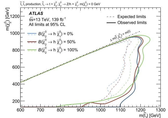
Fig. 11 Exclusion limits at 95% CL on the masses of the \tilde{t}_1 and \tilde{\chi}_2^0 , for a fixed m(\tilde{\chi}_1^0) = 0 GeV and different values of B(\tilde{\chi}_2^0 \rightarrow h\tilde{\chi}_1^0) with B(\tilde{\chi}_2^0 \rightarrow Z\tilde{\chi}_1^0) = 1 - B(\tilde{\chi}_2^0 \rightarrow h\tilde{\chi}_1^0) . The dashed and solid lines are the expected and observed limits for the central value of the signal cross-section, respectively. The expected and observed limits do not include the effect of the theoretical uncertainties in the signal cross-section
