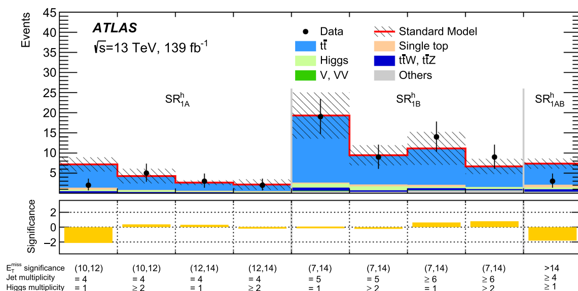
Fig. 9 Comparison of the observed and expected event yields in all the 1\ell SRs and bins used for the model-dependent exclusion limits. The ‘Higgs’ category contains the contributions from gluon–gluon fusion, vector-boson fusion, Wh , Zh and t\bar{t}h production. The ‘Others’ category
