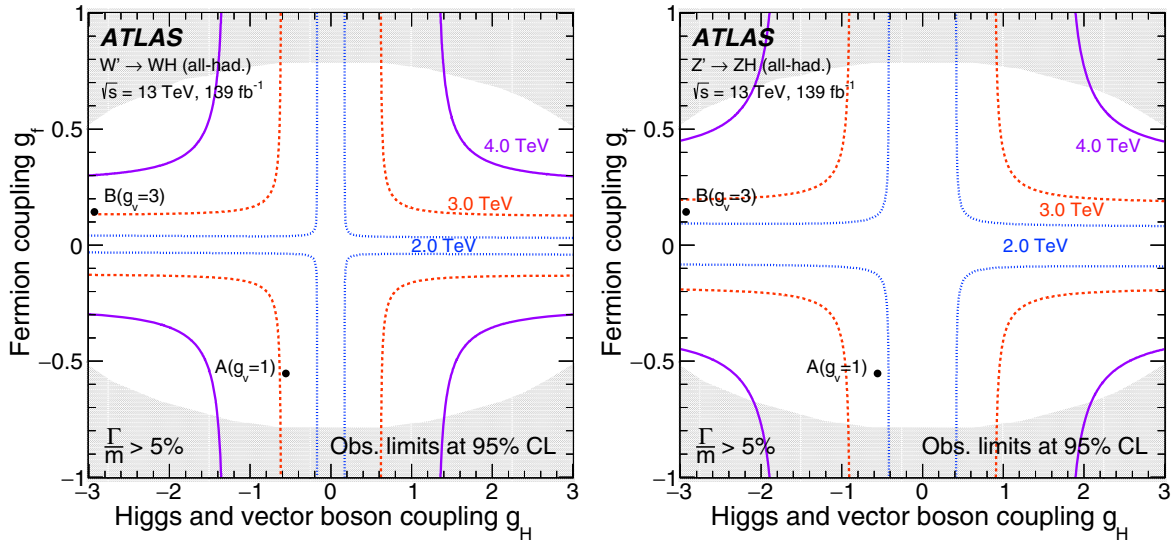
FIG. 7. Limits at 95% C.L. in the g_f vs g_H plane for resonance masses of 2, 3, and 4 TeV for the WH (left) and ZH (right) channels in the context of the HVT model. The coupling values corresponding to HVT models A and B are indicated by filled circles. The gray region indicates values of the couplings corresponding to V' resonances with \Gamma/m greater than 5%. In that region, the assumption that the V' signal m_{JJ} shape is dominated by the experimental resolution is no longer valid.
