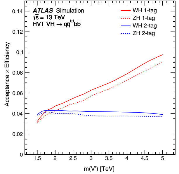
FIG. 2. Signal acceptance times efficiency as a function of the resonance mass, for events in the WH (solid lines) and ZH (dashed lines) signal regions, in the 1-tag and 2-tag categories, with respect to the total number of generated events in each sample. The HVT MC samples include only V' \rightarrow VH decays with V \rightarrow q\bar{q}^{(b)} and H \rightarrow b\bar{b} or c\bar{c} .
