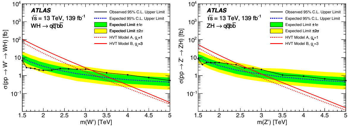
FIG. 6. Observed and expected 95% C.L. upper limits on the cross section for pp \rightarrow V' \rightarrow VH in the WH (left) and ZH (right) channels. The solid (dashed) lines show the cross-section predictions as a function of the resonance mass in the context of HVT model B (A).
