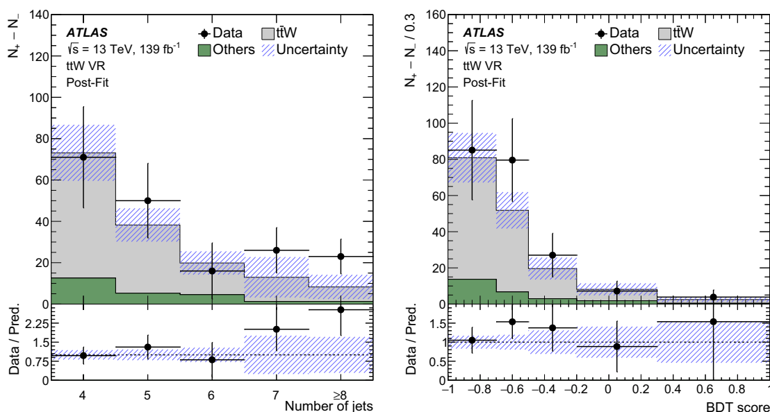
Fig. 5 Post-fit comparison between data and prediction in the t\bar{t}W +jets validation region for the multiplicity of jets (left) and the BDT score (right). The y-axis label N_+ - N_- represents the difference between the number of events with a positive sum and the number of events with a
